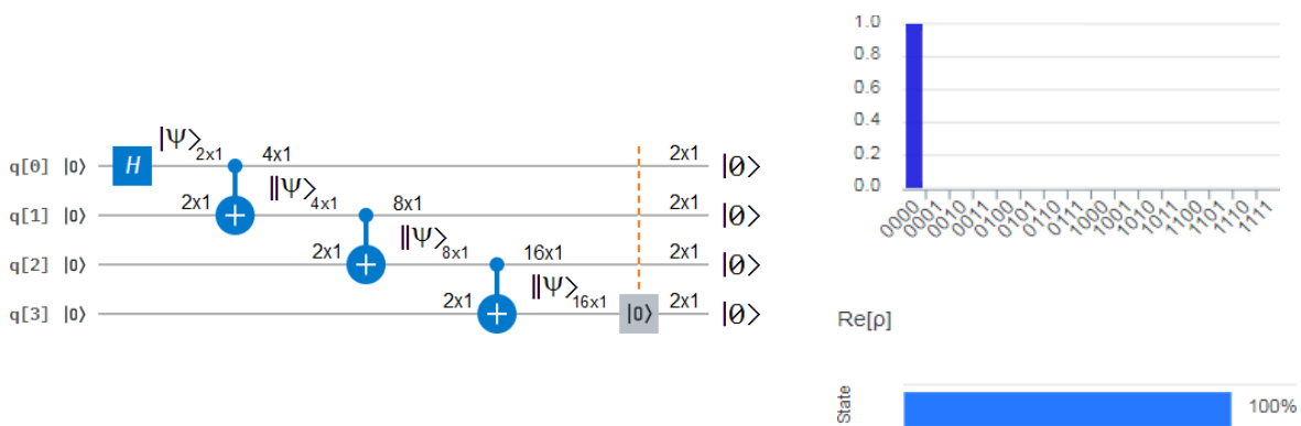
Figure 75 On the left, the configuration starts with the generation of the state |+\rangle , the first CNOT gate generates an EPR pair, while the following ones produce successive stretching of the pair. The qubit reset gate in the lowest branch put all the output to ground state |0\rangle . On the top-right is the unitary wavefunction's complex modulus, and on the bottom-right is the real part of the state, which is unitary too.
