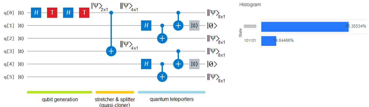
Figure 91 Identical considerations about the previous cases, but the use of a simplified version of the teleporters generates more stretching at the output of the configuration.
