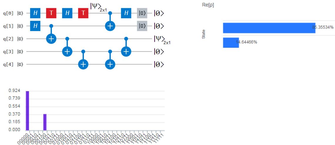
Figure 71 On the top-left is the quantum circuit for controlled quantum teleportation where the lower branch of the EPR pair is stretched twice and shrunk twice, annull their effects mutually. On the bottom-left, the height of the bar is the complex modulus of the wavefunction. Finally, on the right is the real part of the state.
