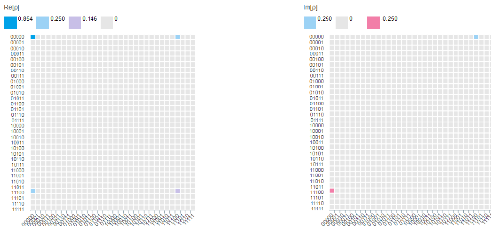
Figure 68 Wavefunction's density matrix: on the left, the real part, and on the right, the imaginary part.
