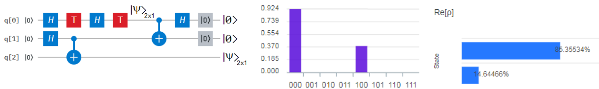
Figure 41 On the left is the quantum circuit for the qubit generation in q[0] and the BSC in q[0] and q[1] . In the middle, the height of the bar is the complex modulus of the wavefunction. On the right is the real part of the state (histogram o measurement probabilities).
