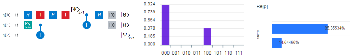
Figure 51 On the left is the quantum circuit for controlled quantum teleportation. In the middle, the height of the bar is the complex modulus of the wavefunction, which is identical to that of Figure 41 . On the right is the real part of the state, also identical to that of Figure 41 .
