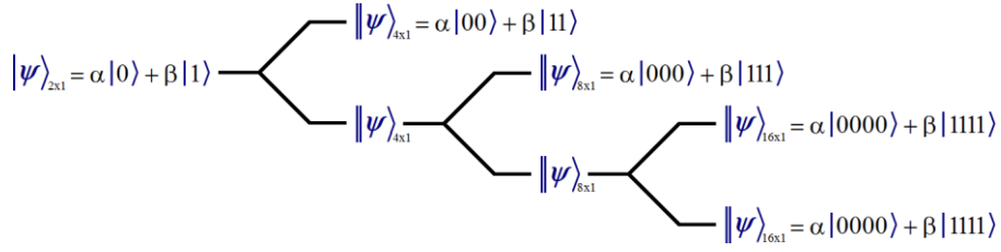
Figure 8 Stretching of the wavefunction by the action of a CNOT gate cascade.
