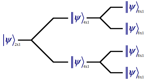
Figure 92 Graphic representation of the rule of inverse-of-the-sizes conservation for this experiment.
