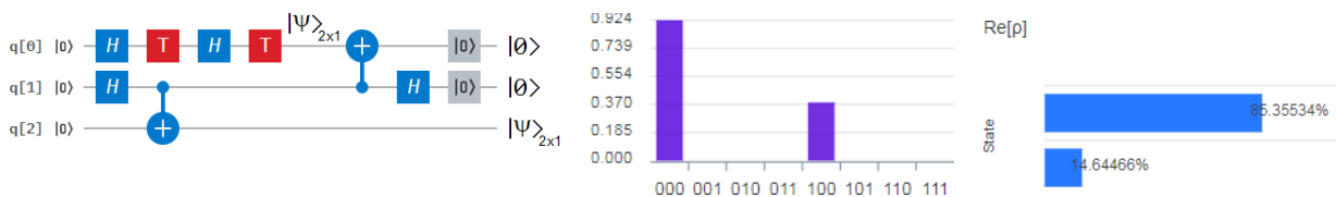
Figure 43 On the left is the quantum circuit for the qubit generation and the swapped BSC between q[0] and q[1] . In the middle, the height of the bar is the complex modulus of the wavefunction. On the right is the real part of the state (histogram o measurement probabilities).
