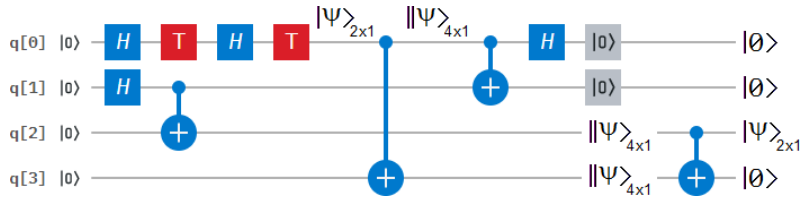
Figure 86 With a similar scheme to the previous case, the final CNOT gate at the output between qubits q[2] and q[3] restores the original qubit to be teleported, and without the need to measure it so as not to alter it, instead, we measure q[3] and depending on how similar it is to a |0\rangle , it is indirectly but with total accuracy that we evaluate the quality of teleportation.
