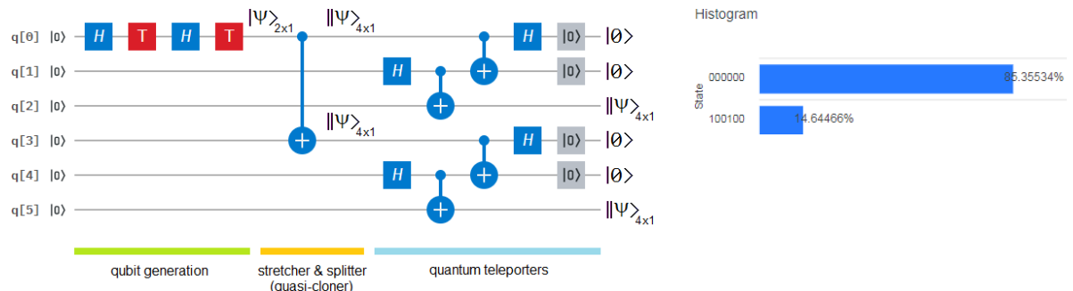
Figure 89 On the left, the quantum circuit for this experiment, which begins with the qubit generation, continue with a quantum stretching where each branch go to its respective teleporter. On the right, the histogram with the real part of the state.
