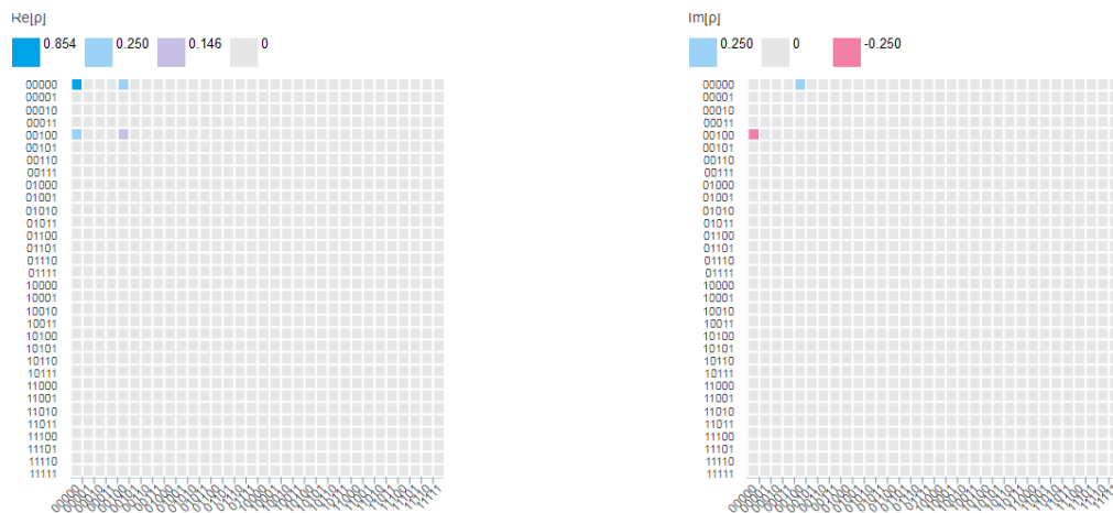
Figure 72 Wavefunction's density matrix: on the left, the real part, and on the right, the imaginary part.
