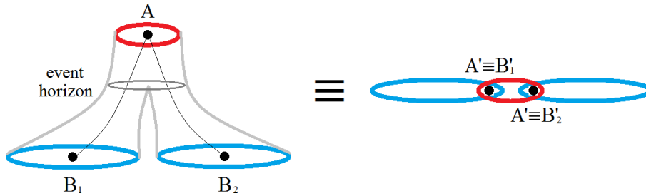
Figure 66 Equivalent wormhole to controlled quantum teleportation with stretching as that of Figure 64 . The stretched quasi-copies of the state to be teleported travel by both branches of the wormhole. From avatars, this wormhole is equivalent to three overlapped rings, being perfectly traversable.
