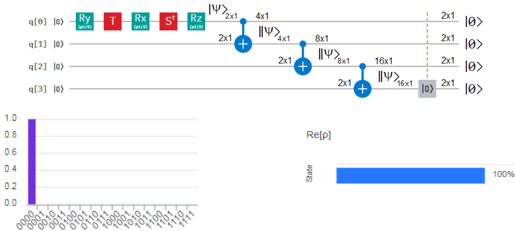
Figure 77 On the top, the generation of a not maximally entangled pair, then, appear two successive CNOT gates in cascade. The presence of a qubit reset gate |0\rangle in the lowest branch simultaneously produces an automatic collapse of all the outputs to the ground state |0\rangle , destroying the stretching and the quasi-entanglement. Finally, the bottom-left, shows a unitary wavefunction's complex modulus, while, bottom-right, shows the real part of the state, which is unitary too.
