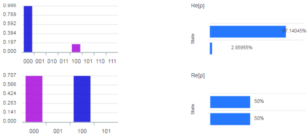
Figure 56 IBM Q delivers two types of outcomes in a randomly way, top: the wavefunction's complex modulus and the real part of the state with different values from those waiting, and, bottom: wavefunction's complex modulus and the real part of the state, but with different values from those waiting again.
