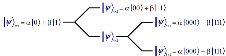
Figure 26 Stretching of the wavefunction by the action of a cascade of CNOT gates.
