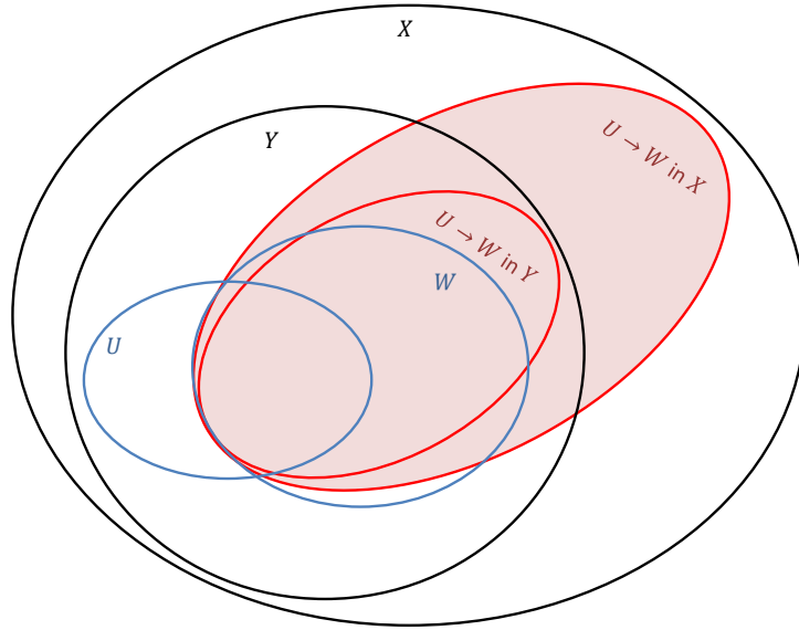
Figure 2: Illustration of what may happen when comparing the exponentials of a topological space with one of its subspaces. Here, Y is a topological subspace of X , U and W are open subsets of Y (and thus of X ), and the exponential U \rightarrow W in Y could be the exponential (U \rightarrow W)_X \cap Y where (U \rightarrow W)_X is the exponential in X .
