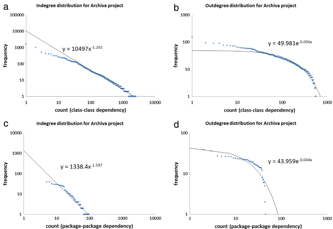
Fig. 7. Double Log degree distribution a. indegree for class–class dependency (top-left) b. outdegree for class–class dependency (top-right), c. indegree for package–package dependency (bottom-left), d. outdegree for package–package dependency (bottom-right).
