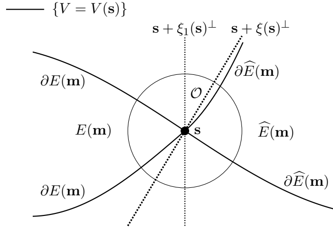
FIGURE 4.1. Representation of the Morse function V near \mathbf{s} \in \mathbf{j}(\mathbf{m}) . Here, \xi_1(\mathbf{s}) denotes an eigenvector of \text{Hess } V(\mathbf{s}) associated with its negative eigenvalue and B^*(\mathbf{s})\xi(\mathbf{s}) \neq 0 . Note that according to the last item in Lemma 1.8, \mathbf{s} + \xi_1(\mathbf{s})^\perp and \mathbf{s} + \xi(\mathbf{s})^\perp coincide if and only if B^*(\mathbf{s})\xi(\mathbf{s}) = 0 .
