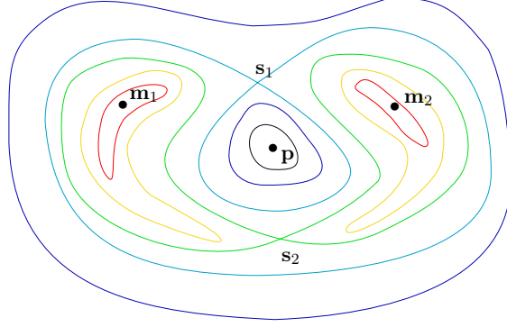
FIGURE 1.1. Some level sets of a Morse function V such that V(x) \rightarrow +\infty when |x| \rightarrow +\infty and admitting five critical points: two local minima \mathbf{m}_1 and \mathbf{m}_2 , one local maximum \mathbf{p} , and two saddle points \mathbf{s}_1 and \mathbf{s}_2 . The point \mathbf{s}_1 is non-separating, whereas \mathbf{s}_2 is separating.
