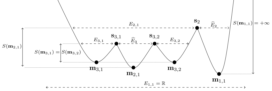
FIGURE 1.3. A 1-D example when V admits four local minima and satisfies Assumption 4. Here, V(\mathbf{m}_{1,1}) < V(\mathbf{m}_{2,1}) < V(\mathbf{m}_{3,1}) = V(\mathbf{m}_{3,2}) , \mathbf{j}(\mathbf{m}_{2,1}) = \{\mathbf{s}_2\} , \mathbf{j}(\mathbf{m}_{3,1}) = \{\mathbf{s}_{3,1}\} , and \mathbf{j}(\mathbf{m}_{3,2}) = \{\mathbf{s}_{3,2}\} . Moreover, \widehat{E}_2 and \widehat{E}_3 denote respectively the sets \widehat{E}(\mathbf{m}_{2,1}) and \widehat{E}(\mathbf{m}_{3,1}) = \widehat{E}(\mathbf{m}_{3,2}) introduced in Remark 1.7.
