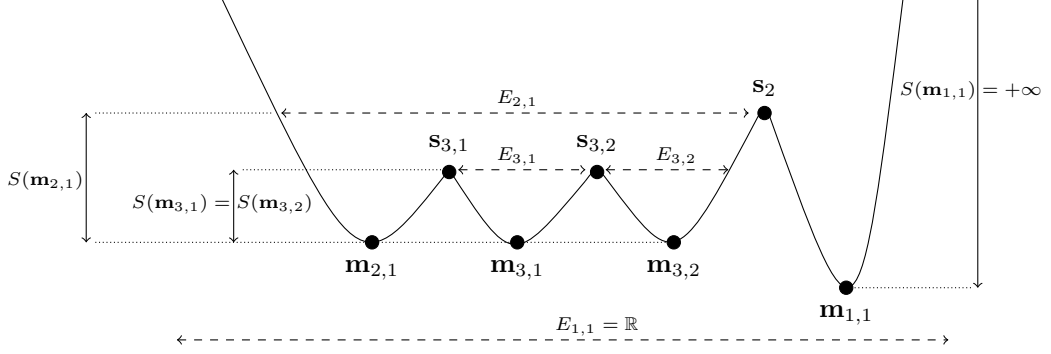
FIGURE 1.2. A 1-D example of the preceding labelling when V admits four local minima. In this example, it holds V(\mathbf{m}_{1,1}) < V(\mathbf{m}_{2,1}) = V(\mathbf{m}_{3,1}) = V(\mathbf{m}_{3,2}) , \mathbf{j}(\mathbf{m}_{2,1}) = \{\mathbf{s}_2\} , \mathbf{j}(\mathbf{m}_{3,1}) = \{\mathbf{s}_{3,1}, \mathbf{s}_{3,2}\} , and \mathbf{j}(\mathbf{m}_{3,2}) = \{\mathbf{s}_{3,2}\} . Note moreover that other choices of construction of the maps \mathbf{j} and E are possible here since \operatorname{argmin}_{E_{2,1}} V = \{\mathbf{m}_{2,1}, \mathbf{m}_{3,1}, \mathbf{m}_{3,2}\} .
