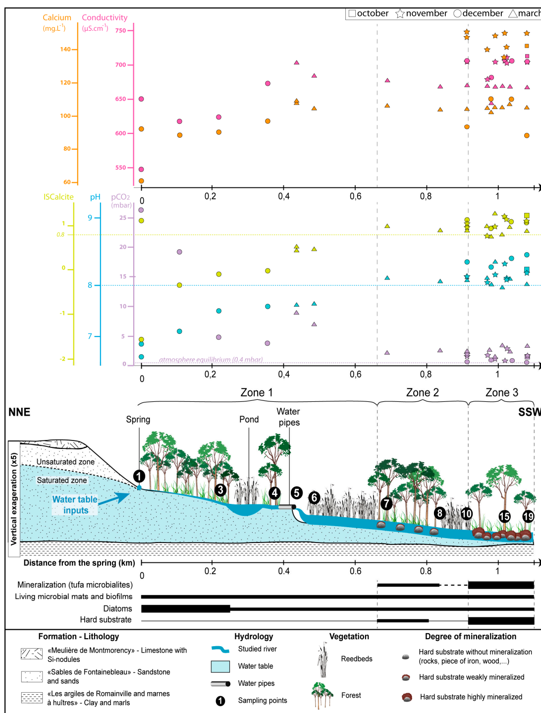
Figure 2. 2D profile of stream showing main hydrochemical characteristics (IS calc ; pH; pCO 2 ; calcium concentration; conductivity; the color of symbols corresponds to the color of the axes of the various hydrochemical variables and shapes of the symbols show the time of the year; mapping of biological (type of vegetation, microbial mats and biofilms, diatoms) and sedimentary (tufa microbialites, hard substrate) characteristics all along the stream.
