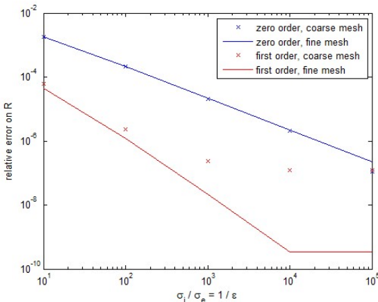
Fig. 2: Convergence of the asymptotic approach at the zero and first orders for two different meshes
