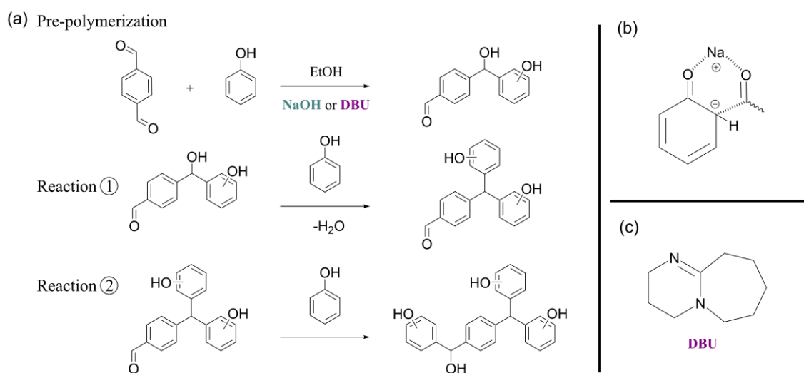
Scheme 1. (a) Mechanism pathway of the reaction between phenol and terephthalaldehyde with the presence of a base, NaOH or DBU. (b) Chelation of methylol and phenoxide by \text{Na}^+ . (c) Chemical structure of 1,8-diazabicyclo[5.4.0]undec-7-ene (DBU).
