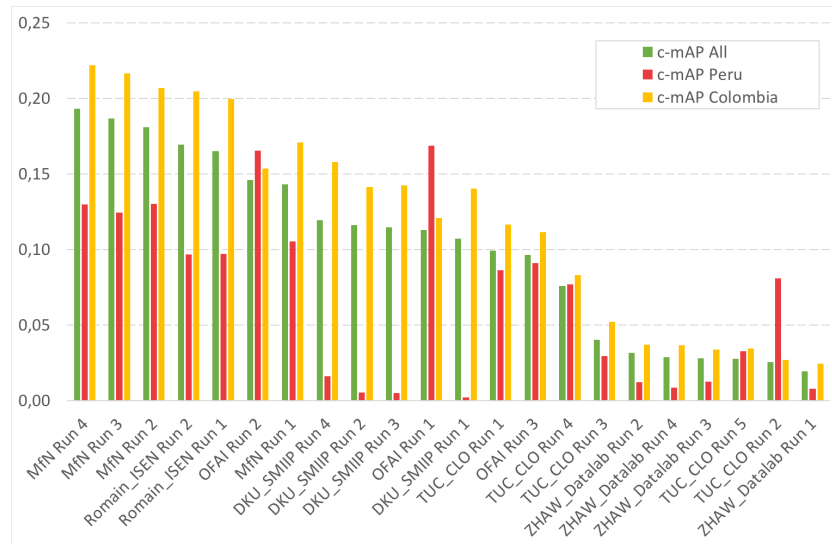
Fig. 3. BirdCLEF 2018 soundscape identification results detailed per country - classification Mean Average Precision.
