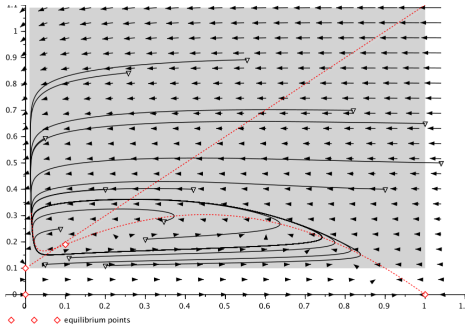
Figure 2: A phase portrait of (1.2) with an unstable equilibrium and a stable limit cycle.
