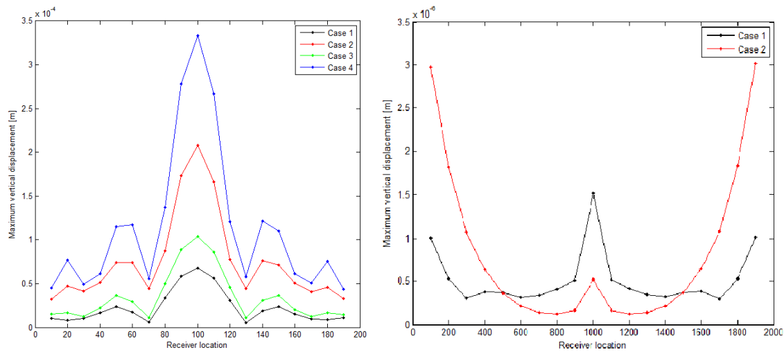
Figure 9. Variations of peak displacements along the profile, for a 100 m radius and 1 km radius (Harmonic source).
