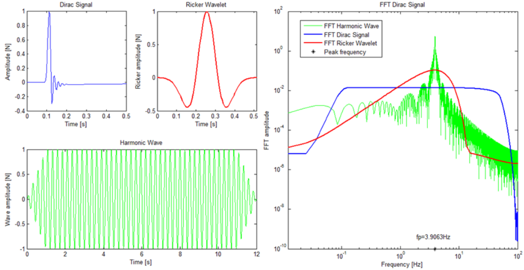
Figure 6. The different sources used in the time domain and their Fourier Transform in a log-log scale.
