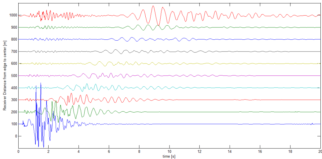
Figure 5. Time domain impulsive response along the profile of ten receivers (from edge to center) for case 2 (low velocity) and for 1 km radius case.
