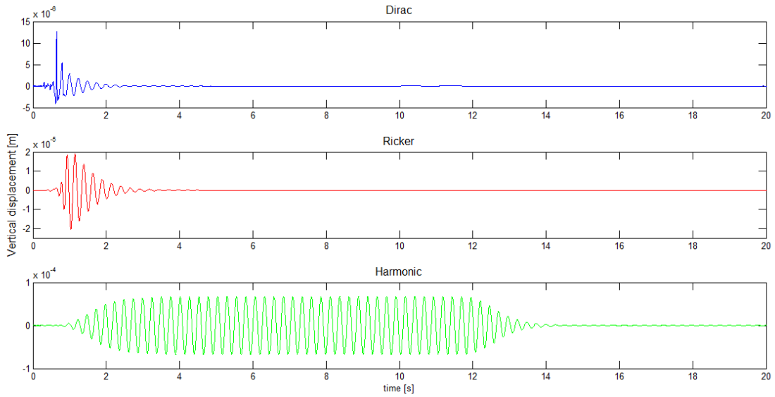
Figure 7. Time domain responses for a Dirac, Ricker and harmonic sources at 100 m radius, at the central receiver for case 1.
