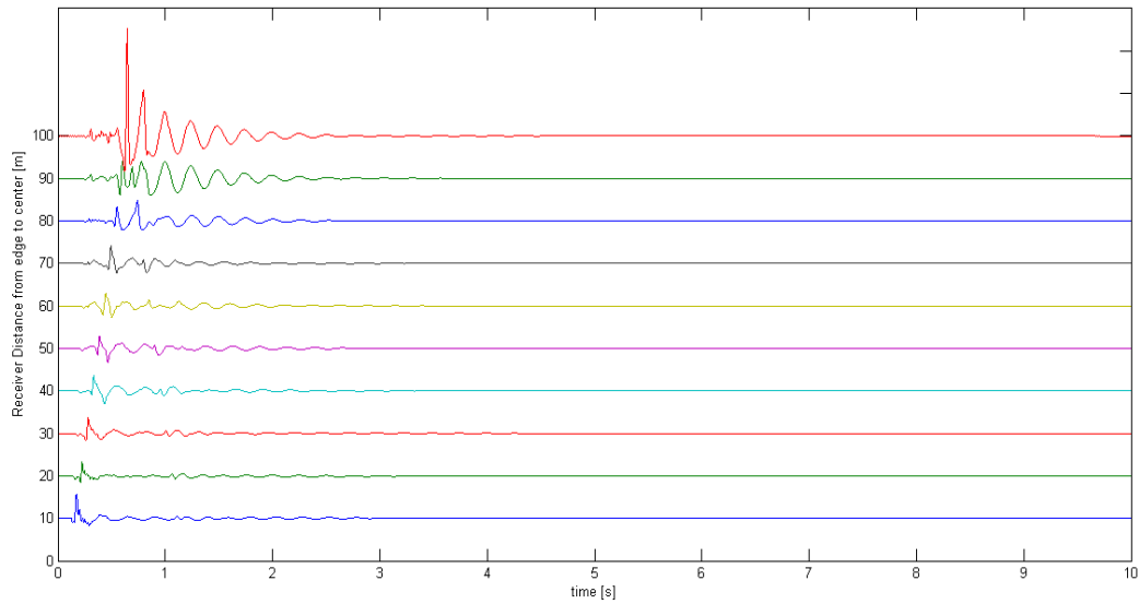
Figure 4. Time domain impulsive response along the profile of ten receivers (from edge to center) for M2.1 soil model and for 100 m radius case.
