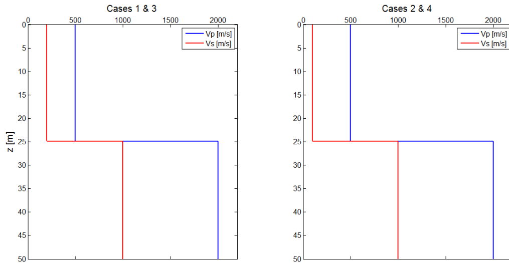
Figure 2. Velocity profile for P and S waves for the soil models.
