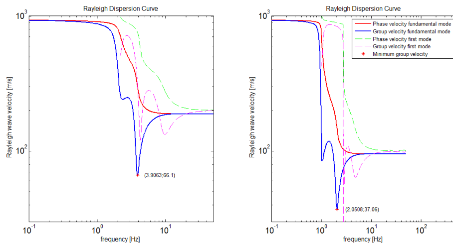
Figure 3. Rayleigh dispersion curves for cases (1+3) and (2+4).
