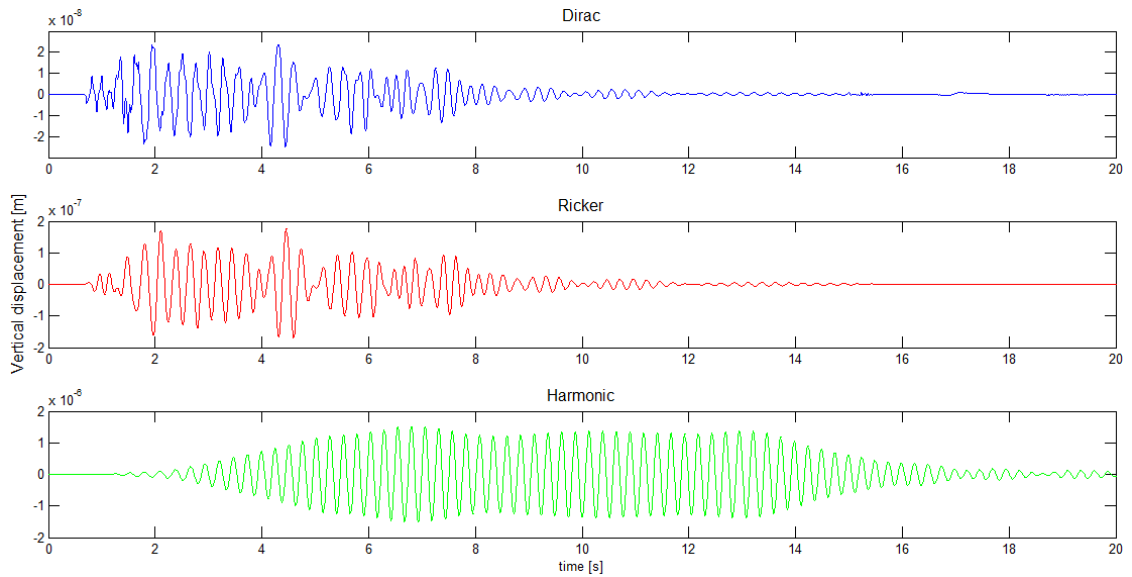
Figure 8. Time domain responses for a Dirac, Ricker and harmonic sources at 1 km radius, at the central receiver for case 1.
