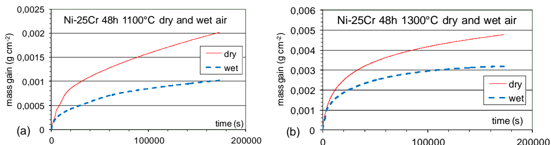
FIGURE 1. Thermogravimetry curves obtained at 1100°C (a) and at 1300°C (b) for the Ni-25Cr alloy in dry air and in wet air, showing the dependence of mass gain on the presence of water vapour
