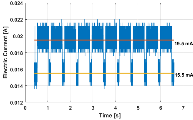
Figure 4. Electric current consumption of the OFDM-EIS system during 10 complete measurements separated by an idle of 100ms.
