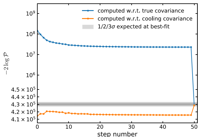
FIG. 3. The posterior probability after each iteration of our algorithm during the run on the simulated dataset described in Sec. V. The top (blue) line is the posterior with respect to the true covariance, and the bottom (orange) line is with respect to the cooling covariance (note the y-scale is mixed log and linear). For the final step these two are identical since the cooling covariance is fully cooled and equals the true covariance. The grey band represents the value of the posterior probability expected at the best-fit point, and our best fit sits well within this expectation.
