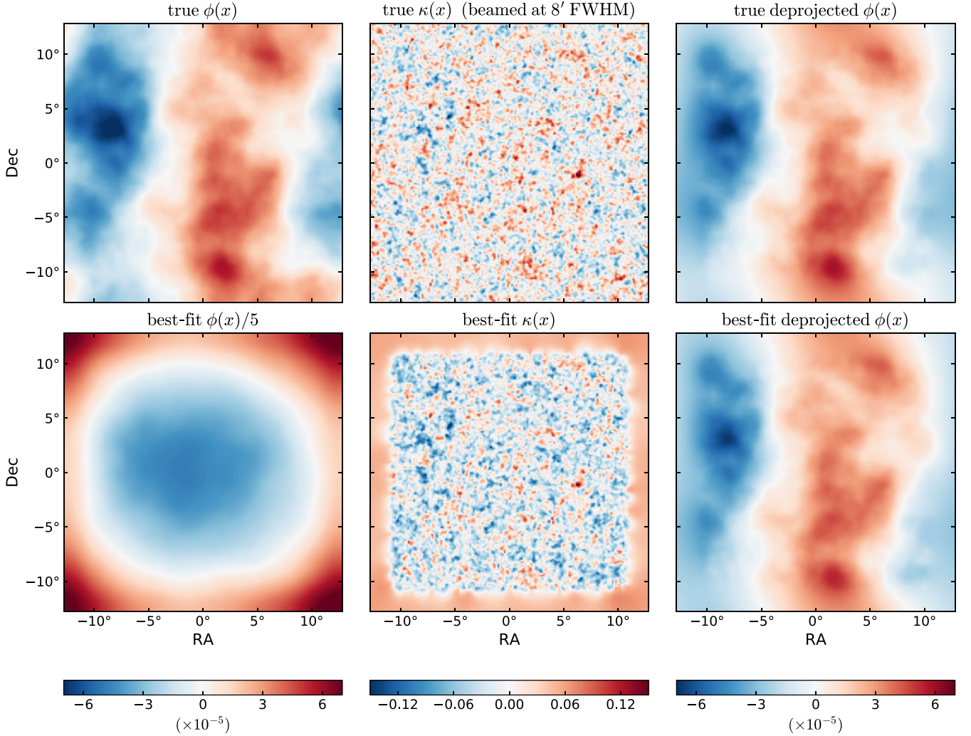
FIG. 6. The reconstructed lensing potential from a run of our algorithm on simulated data (bottom row), as compared to the simulation truth (top row). The first column is the raw \phi(x) map that maximizes the posterior. The middle column is the corresponding convergence, \kappa(x) \equiv -\nabla^2\phi(x)/2 , which allows one to see the good agreement with the truth in the unmasked regions. A small uniform negative “mean-field” correction inside the mask is visually recognizable as a slight preponderance of blue. The final column is after deprojecting this mean field using the procedure described in Sec. V B, allowing one to better recognize the agreement with the true \phi map.
