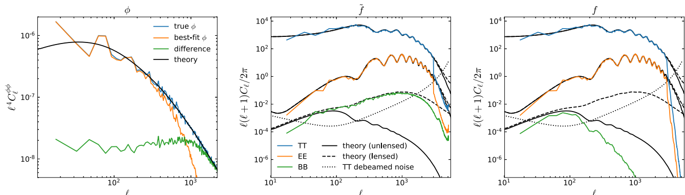
FIG. 2. The power spectra of the best-fit \phi and lensed/unlensed CMB maps from a run of our algorithm, as compared to the input theory spectra. This is for the run with only Fourier-space masking described in Sec. V A (the same run for which maps are shown in Fig. 1). The left panel also shows the power spectrum of the simulation truth for the \phi map itself as well as the power spectrum of the difference between this and our reconstructed solution, demonstrating the fidelity of the reconstruction. The “bump” visible in the lensed spectra near the Nyquist frequency at \ell = 3600 signals the smallest scale for which the LenseFlow pixelized lensing approximation is accurate at this pixel size (similar features are produced by other lensing algorithms). We mask the data in Fourier space beyond \ell = 3000 so that we are not sensitive to this region, and the effects of this mask are visible above as a sharp suppression in power at \ell > 3000 . Note: The beam-deconvolved noise spectrum shown in the middle and right panel are used to illustrate the effective signal-to-noise ratio in the simulated data. The actual simulation data used to generate the best-fit \phi and lensed/unlensed CMB maps are not beam-deconvolved. See Sec. V for details.
