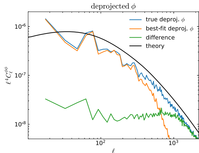
FIG. 7. The power spectra of the best-fit \phi map as compared to the simulation truth and theory spectrum for the run with real-space masking described in Sec. VB. The best fit and simulation truth \phi maps are the ones shown in the right column of Fig. 6 and have had the mean-field deprojected according to the procedure described in Sec. VB.
