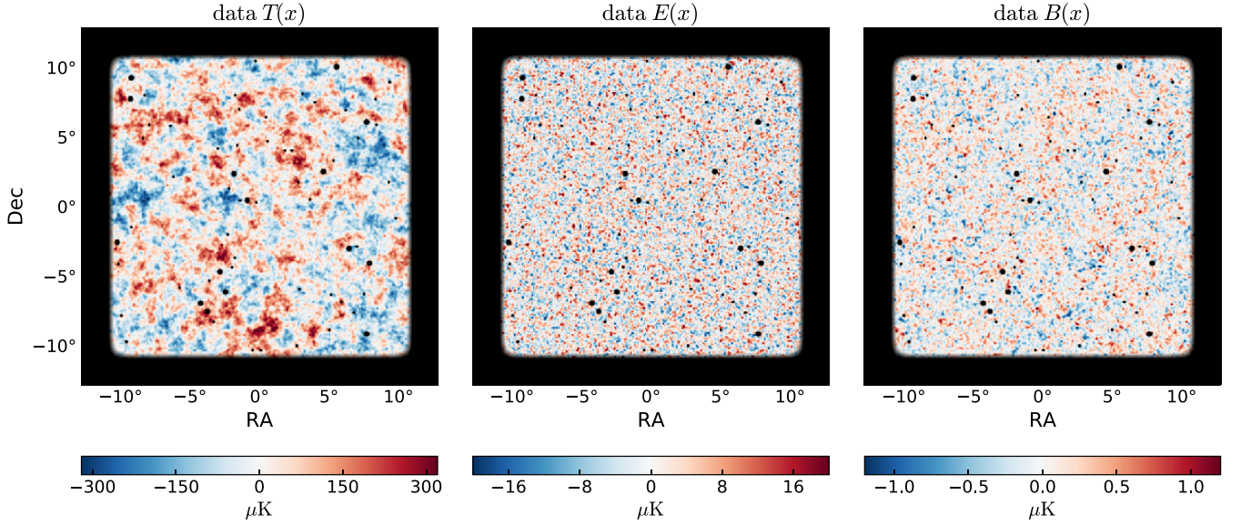
FIG. 4. The simulated data used in the runs described in Sec. V. We use a 512 \times 512 grid with 3 arcmin pixels, which covers roughly 600 \text{ deg}^2 . It assumes a setup approximating an expected CMB-S4 configuration, with a 3 arcmin beam and stationary 1 \mu\text{K} -arcmin temperature noise, modulated to include a 1/f contribution below \ell_{\text{knee}} = 100 (see text for more details). One hundred unapodized point sources with radii between 5 and 10 arcmin are randomly placed within the region. A 2^\circ mildly apodized border mask is applied, as well as a Fourier-space cut above \ell > 3000 . Note that for this figure the mask is simply overlaid on the unmasked T , E , and B images rather being multiplied into T , Q , and U as is done in the likelihood, since multiplying it in would result in large E to B leakage spoiling the ability to see B . Additionally, the unmasked data has been Wiener filtered with the lensed CMB covariance as the signal covariance to reduce the visual impact of noise.
