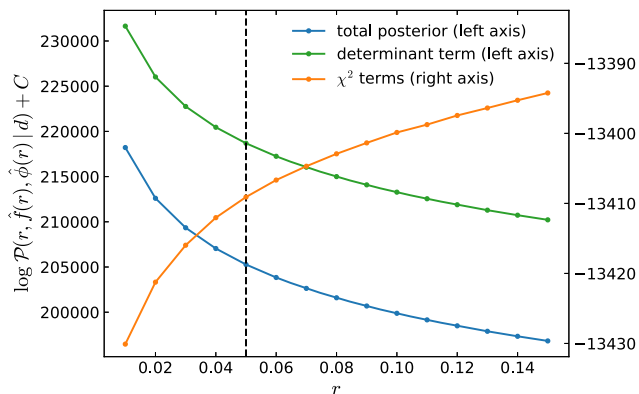
FIG. 9. A slice through the joint posterior probability (3), varying r and maximizing with respect to f and \phi for each value of r . For speed, we have reduced the map size as compared to the main runs described in this work to 128 \times 128 pixels (while keeping the relative width of the border mask the same). The green curve (left axis) is the contribution from \det C_f(\theta) , the orange curve (right axis) is the contribution from the three \chi^2 terms [i.e., the first three terms of (3)], and the blue (left axis) is the sum of these two. This demonstrates that the joint MAP estimate of r is not useful as it is driven to zero. The lack of apparent numerical noise in the orange curve demonstrates the stability of the maximization algorithm.
