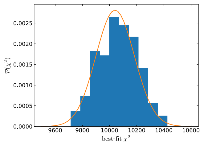
FIG. 8. Distribution of the \chi^2 of the best-fit point from runs on 500 different simulated datasets. For speed, we have reduced the map size as compared to the main runs described in this work to 128 \times 128 pixels (while keeping the relative width of the border mask width) and use only E and B . The expected distribution of the best-fit \chi^2 under a Gaussian approximation of the posterior is shown as the orange curve.
