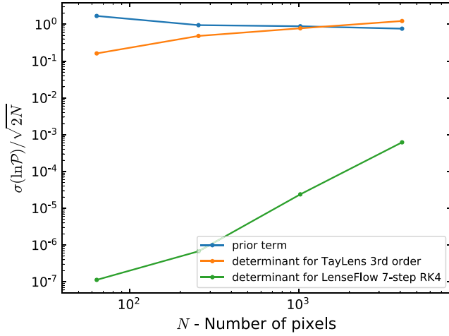
FIG. 11. The standard deviation of the variation in the log probability values for the \phi -prior term, \phi^\dagger \mathbb{C}_\phi^{-1} \phi , and lensing determinant term, 2 \log |\det \mathbb{L}(\phi)| , in (5), as computed from Monte Carlo samples of \phi . These samples approximate samples from the posterior probability \mathcal{P}(f, \phi|d) for some simulated data, d , assuming full-sky temperature-only reconstruction noise. Here we have used 7th order Taylor series lensing on 1 arcmin pixels with temperature-only data. Because the variation in the two terms is of similar order, the determinant cannot be ignored.
