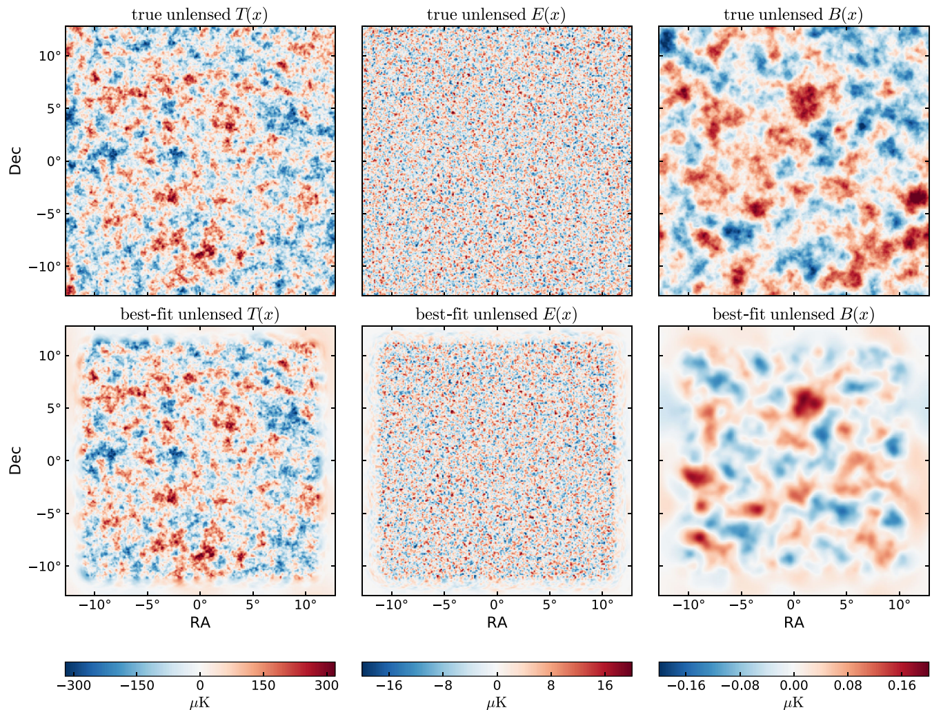
FIG. 5. The reconstructed unensured T , E , and B maps from a run of our algorithm on simulated data (bottom row), as compared to the simulation truth (top row). This is for the run discussed in Sec. VB which includes the real-space mask that is visible in Fig. 4. As expected, low signal-to-noise modes are attenuated and the solution provides a partial reconstruction even in the masked region.
