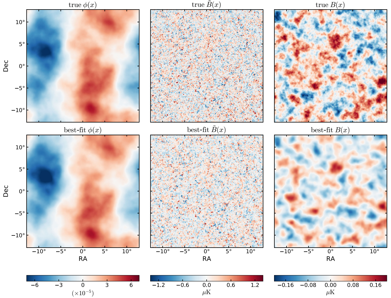
FIG. 1. The reconstructed \phi and lensed/unlensed B maps from a run of our algorithm on simulated data (bottom row), as compared to the simulation truth (top row). This is for the run with only Fourier-space masking described in Sec. VA. The reconstruction, as expected, resembles a Wiener filter solution wherein low signal-to-noise modes are attenuated.
