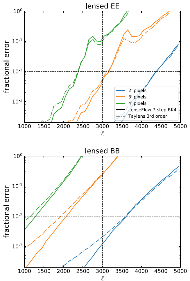
FIG. 10. Comparison of the accuracy of LenseFlow vs Taylor series lensing augmented with a nearest-pixel permutation (i.e., “Taylens” [35]). The quantity plotted is the spectrum of \mathbb{P}\mathbb{L}_{\text{true}}(\phi)f - \mathbb{L}(\mathbb{P}\phi)\mathbb{P}f divided by the theoretical EE or BB spectrum, where \mathbb{P} is a pixelization operation and \mathbb{L}_{\text{true}} is an asymptotically high order LenseFlow. The first term represents the “true” lensed field, while the latter performs lensing on a pixelization map. For the “true” fields, we use pixels 4 times smaller on a side than the pixelized version. This figure demonstrates that our use of 7-step LenseFlow on 3 arcmin pixels incurs an error of \sim 20\% in BB by \ell = 3000 , which is far below the instrumental noise at this multipole for, e.g., CMB-S4. The error is approximately the same as using Taylens, showing that the error is driven by the loss of information due to pixelization rather than due to an error in ODE integration or due to Taylor series truncation.
