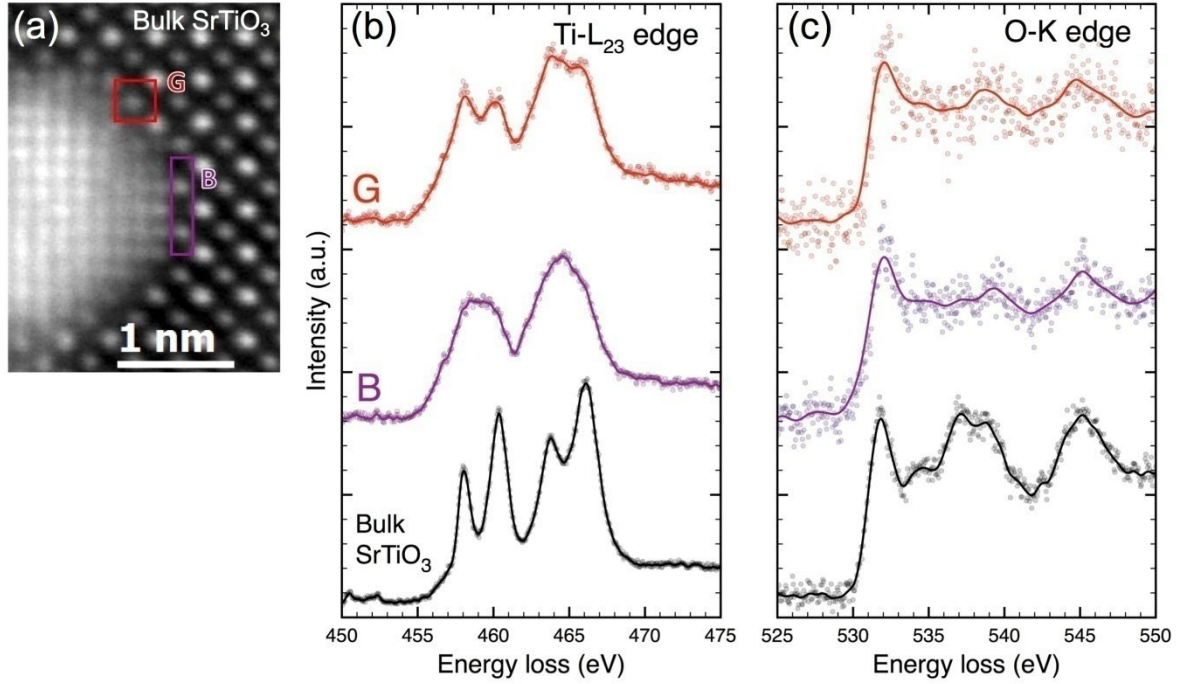
Figure S2. Ti- L_{2,3} and O-K ELNES differences between [100]_{\text{STO}}||[100]_{\text{Ni}} and the [110]_{\text{STO}}||[110]_{\text{Ni}} nanowire-matrix interfaces. While the crystal-field splitting is almost completely lost in B due to the symmetry breaking at the interface and the covalent interaction with neighboring Ni atoms, it is still partially visible in G where the Ti local environment is slightly less affected by the interface. The O-K edge still shows the fingerprint of the hybridization with the Ti-3d states but the spectral weight of the higher lying Sr-4d states is strongly reduced in B and G compared to bulk STO. The points correspond to the experimental data while the lines are just guides for eye.
