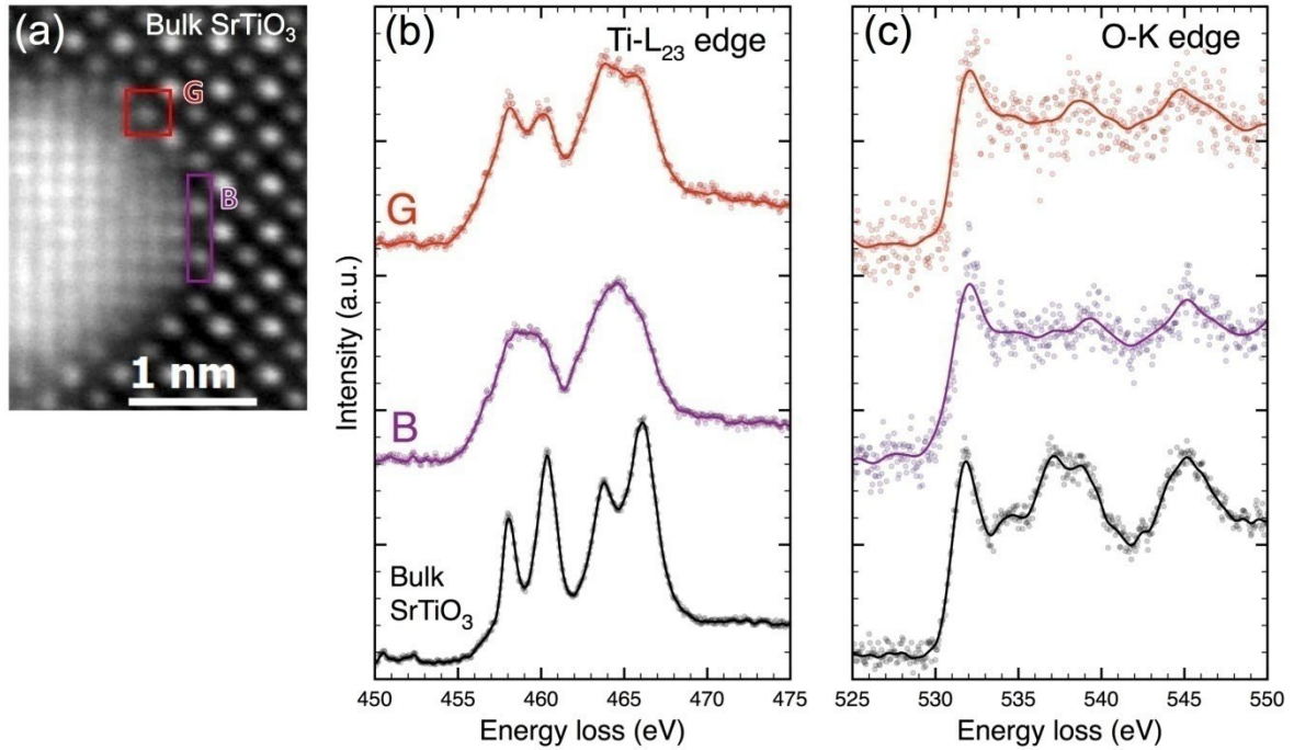
Figure S2. Ti- L_{2,3} and O- K ELNES differences between [100]_{\text{STO}}||[100]_{\text{Ni}} and the [110]_{\text{STO}}||[110]_{\text{Ni}} nanowire-matrix interfaces. While the crystal-field splitting is almost completely lost in B due to the symmetry breaking at the interface and the covalent interaction with neighboring Ni atoms, it is still partially visible in G where the Ti local environment is slightly less affected by the interface. The O- K edge still shows the fingerprint of the hybridization with the Ti- 3d states but the spectral weight of the higher lying Sr- 4d states is strongly reduced in B and G compared to bulk STO. The points correspond to the experimental data while the lines are just guides for eye.
