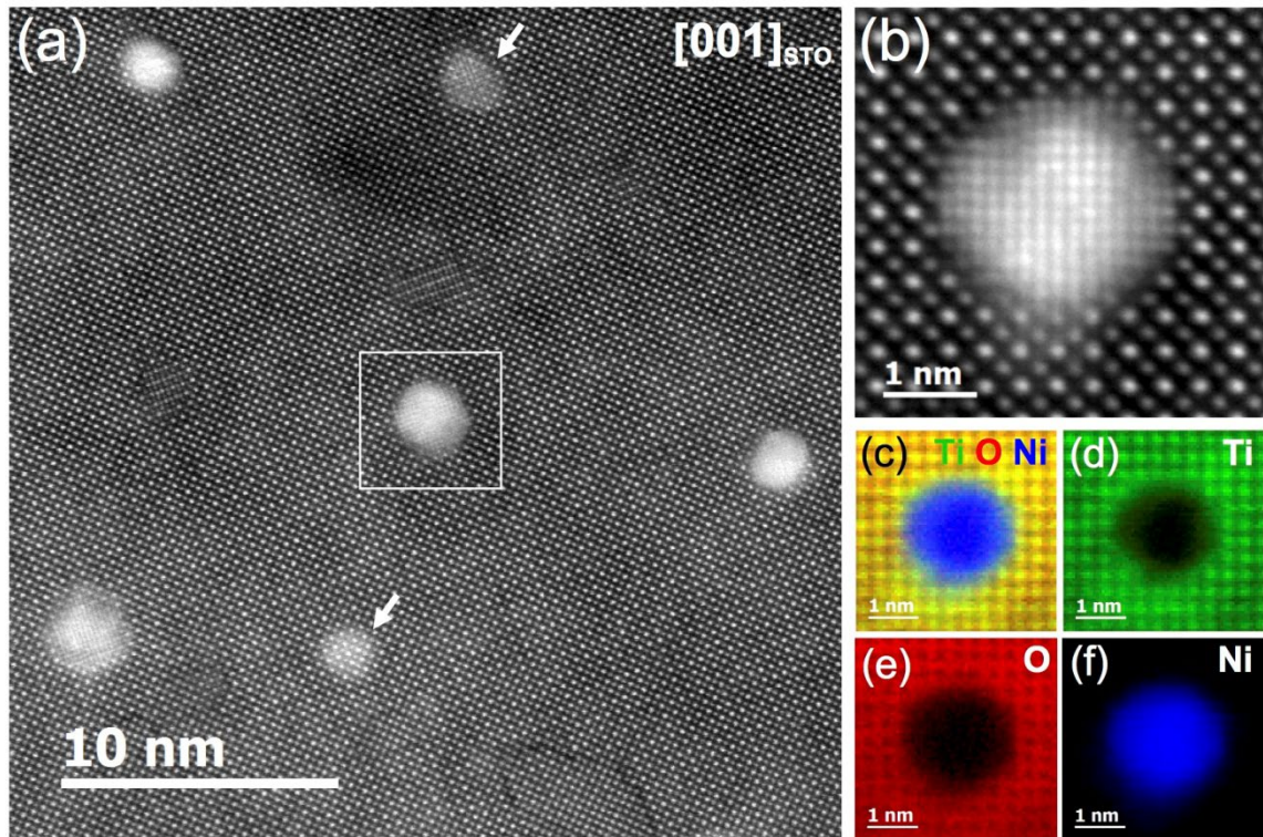
Figure 2. (a) Global HAADF top view, along [001] zone axis, of the sample showing a few Ni nanowires in the STO matrix. The STO and Ni lattices appear superimposed for short nanowires, as indicated by arrows, in which case the top or bottom surface of the thinned sample does not intersect the nanowires. Detailed analysis of a typical nanowire of diameter 2 nm: (b) high-resolution HAADF image obtained after alignment of a stack of 42 images, showing the atomic structure of the nanowire; (c) composite chemical map of the nanowire built from the elemental Ti map shown in (d), O map in (e) and Ni map in (f) extracted from the Ti- L_{2,3} edges ( \sim 457 eV), the O- K edge ( \sim 531 eV) and the Ni- L_{2,3} edges ( \sim 855 eV) respectively. All maps are displayed after noise removal through principal component analysis (PCA). Variations of the intensity with the STO lattice periodicity is visible on the Ti and O maps but not in the Ni nanowire due to the smaller lattice spacing in the metal.
