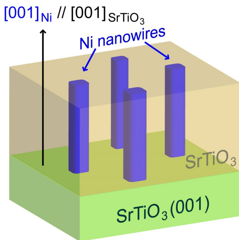
Figure 1. Schematics of a \text{Ni}:\text{SrTiO}_3/\text{SrTiO}_3(001) epitaxial VAN structure.
