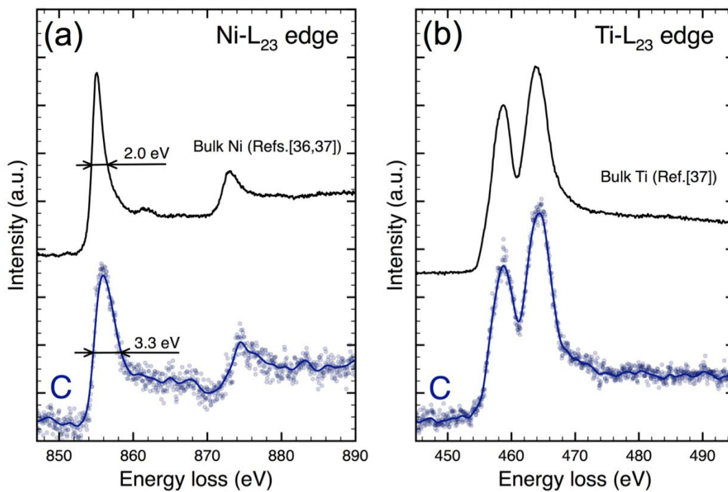
Figure S3. (a) Comparison between (a) the Ni- L_{2,3} and (b) the Ti- L_{2,3} edges obtained at the Ni-STO matrix interface (area C in Figure 3) and reference spectra obtained on bulk Ni and bulk Ti, respectively. The points correspond to the experimental data while the lines are just guides for eye.
