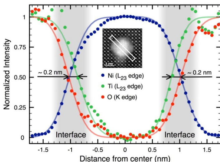
Figure S1. Ni, Ti and O chemical profiles across the nanowire obtained by integrating EELS signal in a box rotated by 45°, as shown in inset. Intensities are normalized to the same maximum height. The same Ti-rich interface can be deduced when comparing the Ti and O profiles and appears as a general feature of the interface. The points correspond to the experimental data while the lines are just guides for eye.
