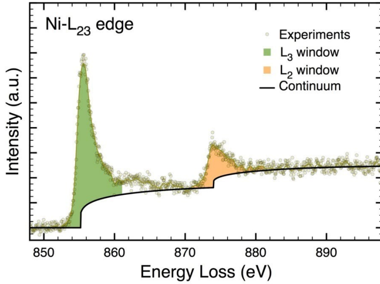
Figure S4. Method employed to extract the Ni- L_3 to L_2 ratio. After removing the background using a power-law fit, the continuum contribution to the edge has been modeled using hydrogenic L cross-sections with a fixed 2:1 ratio for the L_3 and L_2 contributions, respectively. The continuum function strength has been scaled using an energy window located between 890 and 910 eV, and subtracted from the experimental signal. The corrected L_3 and L_2 white-line intensities have been obtained by integrating the signal over the 10 eV wide windows shown in the figure. Points correspond to the experimental data.
