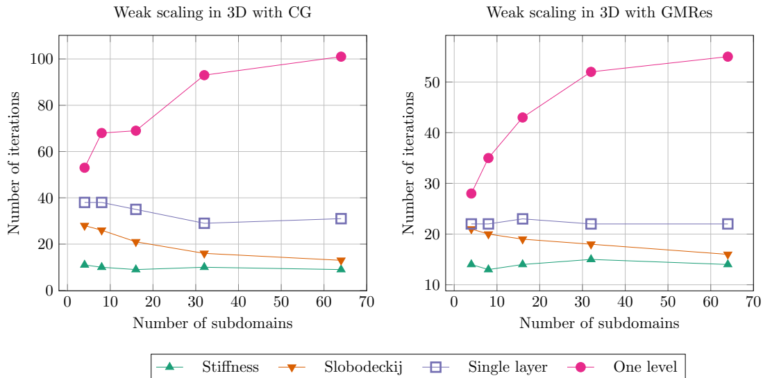
Figure 14: Weak scaling to solve Equation (21) in 3D
