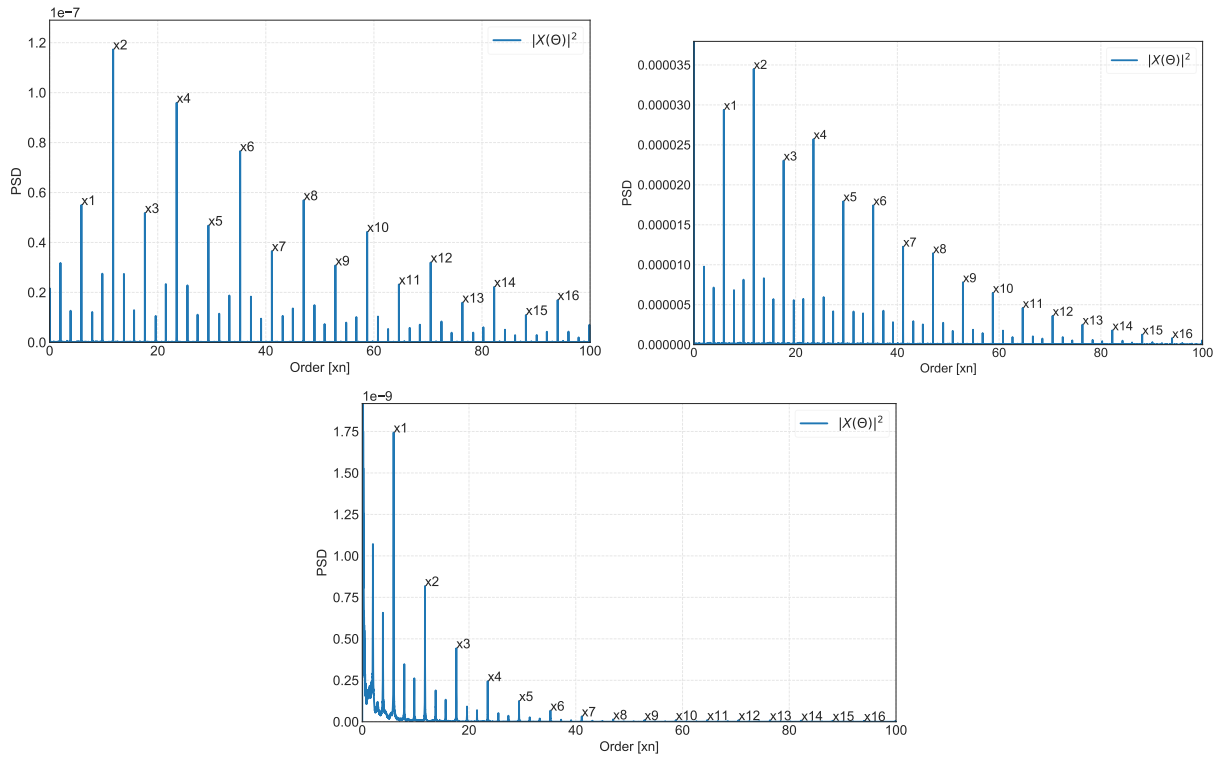
Figure 7: Top-row: baseline methodologies, left) angular domain transform, SK filtering, then envelope spectrum, right) SK filtering, angular domain transform, then envelope spectrum, bottom-row: proposal) angular domain transform, then, envelope spectrum convolved with a time-frequency dependent SK based filter.
