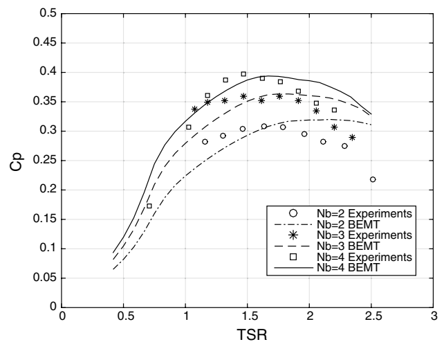
Fig. 14 Power coefficient for BEMT simulations and experiments—with scaling up extrapolation. The error propagation procedure is presented in “Appendix A”
