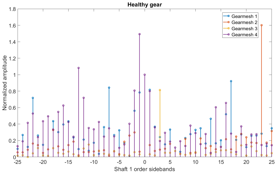
Figure 2. Sideband amplitude patterns of the first 4 gearmesh harmonics. 20 Nm - 20 Hz test.
