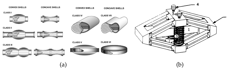
Figure 1: a) Sketch of various classes of flexensional transducers [1, 2]. b) Sketch of a Class IV flexensional piezoelectric transducer. [3]
