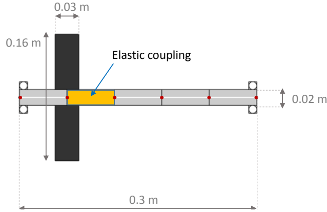
Figure 2: studied rotor
