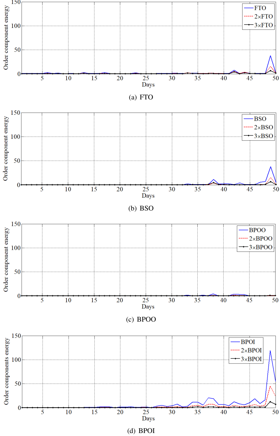
Figure 4 – Evolution of the order component energy for the different type of fault that can occur on the bearing over the 50 days of measurement: (a) cage fault, (b) Rolling elements fault, (c) Outer-race fault and (d) Inner-race fault.
