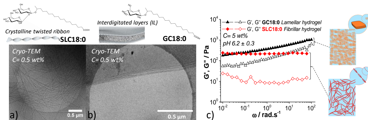
Figure 1 – a-b) Cryo-TEM images of the typical a) fibrillar and b) lamellar structures of SLC18:0 and GC18:0 observed under diluted conditions ( C= 0.5 wt%) and \text{pH } 6.2 \pm 0.3 . c) Angular frequency, \omega , dependence of elastic, G' (closed symbols), and loss, G'' (open symbols), moduli for fibrillar SLC18:0 (red diamonds) and lamellar GC18:0 (black triangles) hydrogels recorded in the linear regime ( \gamma = 0.02\% and 0.05\% , respectively) at \text{pH } 6.2 \pm 0.3 and C= 5 wt% prior to freeze-casting. The drawings show the respective bulk structure of the hydrogels: homogeneously entangled fibers for SLC18:0 and heterogeneous dispersion of interconnected large lamellar domains for GC18:0.
