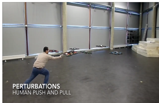
Fig. 13: Experiment with push perturbation
