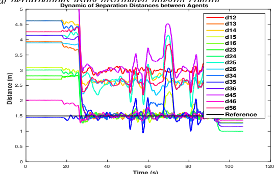
Fig. 12: Experiments: Inter-distances between 6 UAVs in an aggregation scenario with external perturbations using distributed integral control
