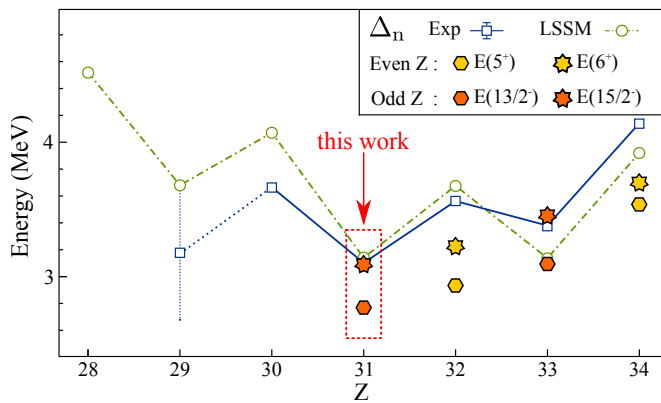
FIG. 4. (Color online) Comparison between the \Delta_n shell gap at N = 50 and the energy of core-excited states in N = 50 isotones. Solid line: \Delta_n from binding energies [28, 48, 49]; Dashed-dotted line: \Delta_n from LSSM calculations; Symbols: excitation energy of core-excited states [47]. The dotted line represents \Delta_n using extrapolated mass for ^{80}\text{Cu} (see text).
