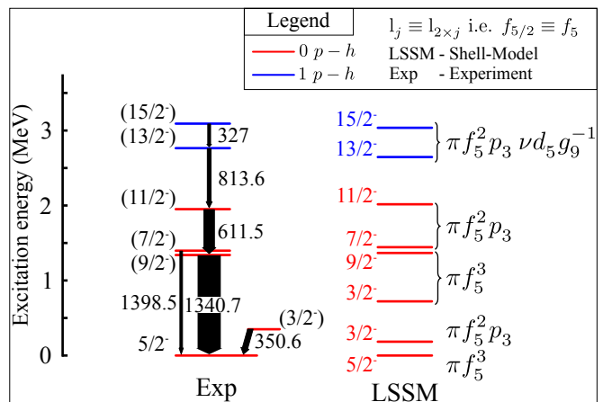
FIG. 3. (Color online) Experimental level scheme observed in the present work (left) and theoretical level scheme (right) of ^{81}\text{Ga} . Levels marked with red (blue) correspond to dominant contributions from 0 p-h (1 p-h) excitations of the ^{78}\text{Ni} core.
