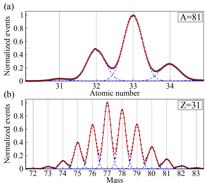
FIG. 1. (Color online) (top) Normalized atomic number distribution for A = 81 isotopes (bottom) Normalized mass distribution for Z = 31 isotopes. The continuous red and dotted blue lines represent respectively the fit of the total distributions and individual mass and atomic charge contributions.
