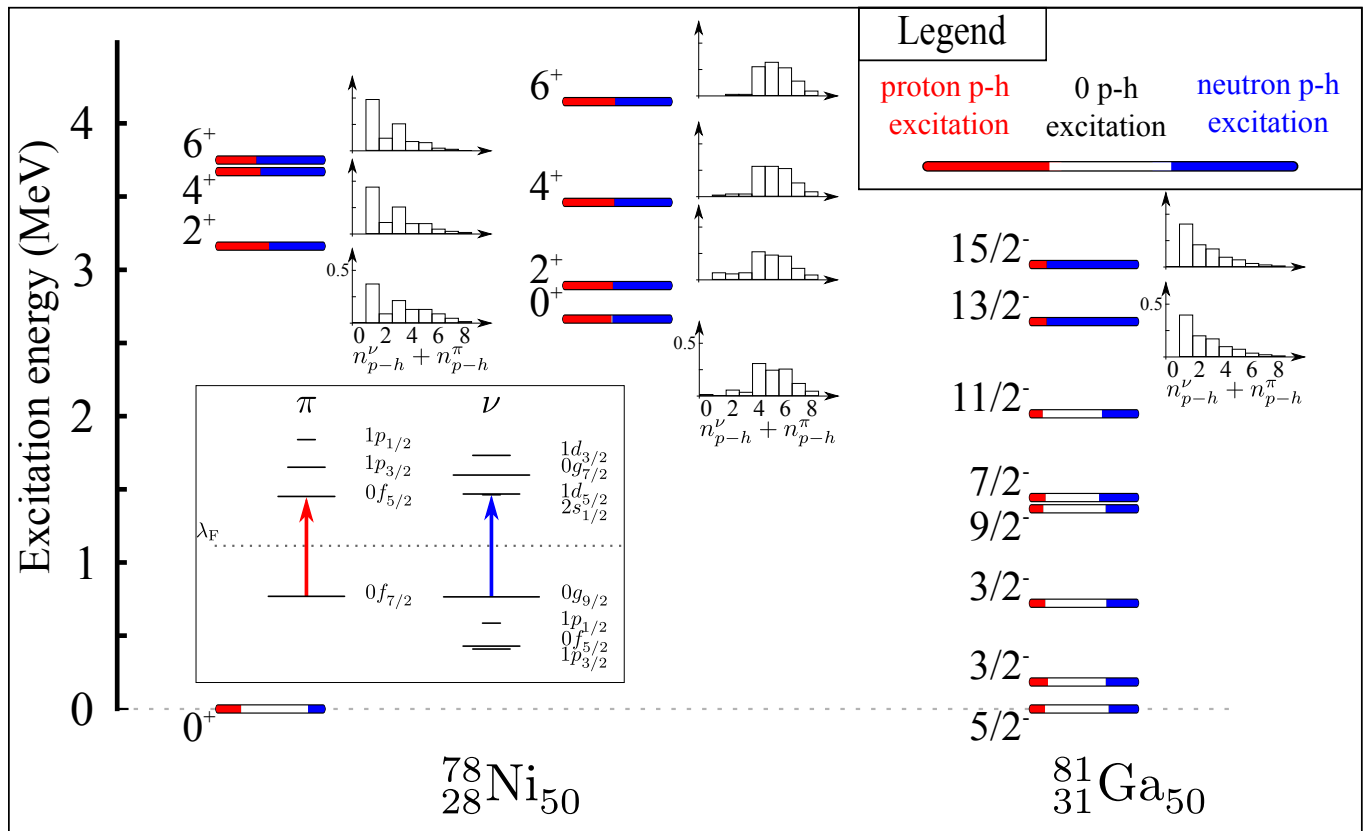
FIG. 5. (Color online) Theoretical predictions for excitation energies and decomposition of the wave functions for states in ^{78}\text{Ni} [11] and ^{81}\text{Ga} (this work). For ^{78}\text{Ni} the spherical (left) and collective (right) states are shown. The histograms represent the distribution of total number of particle-hole excitations of the inert core ( n_{p-h}^{\nu} + n_{p-h}^{\pi} ) contributing to the state. The contribution of the excitations of the inert core due to the protons (red) and neutrons (blue) is represented in color in terms of probability in each level (the length of the color bar is normalized to 100% for each state), the white area corresponds to a closed inert core configuration. The relevant single-particle proton and neutron states are also shown.
