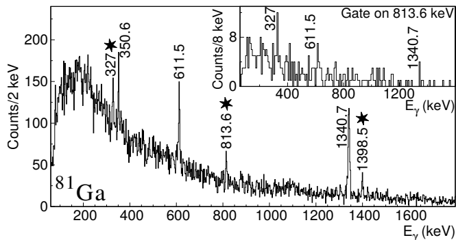
FIG. 2. (Color online) Tracked Doppler corrected \gamma -ray spectrum measured in coincidence with the isotopically identified ^{81}\text{Ga} . Known \gamma -ray transition energies are labeled and newly reported transitions are marked with star symbols. The inset shows the \gamma - \gamma coincidence gated on the 813.6 keV transition in ^{81}\text{Ga} .
