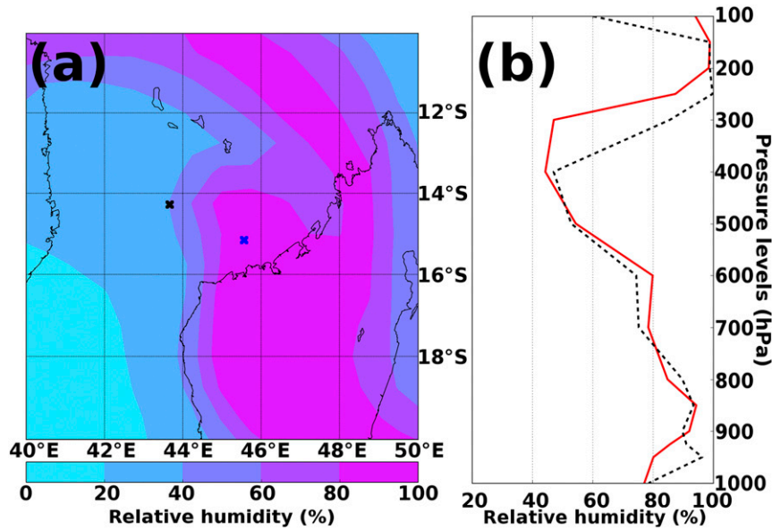
FIG. 2. Spatial and vertical distributions of relative humidities (%) in the environment of VITC Hellen at lead time 24 h (0000 UTC 31 Mar). (a) At 400 hPa from ERA-Interim reanalysis data. The best track TC center is indicated by the blue cross. (b) Vertical profile at the location indicated by the black cross on Fig. 2a from ERA-Interim (red line) and AROME-IO experiment averaged on a 40-km disk in order to compare to the 80-km resolution of the ERA-Interim reanalysis data (dashed black line).
