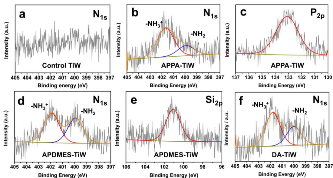
Figure 6. (a) N 1s core level of control TiW. (b) N 1s core level and (c) P 2p core level of APPA-TiW, (d) N 1s core level and (e) Si 2p core level of APDMES-TiW, (f) N 1s core level of DA-TiW.
