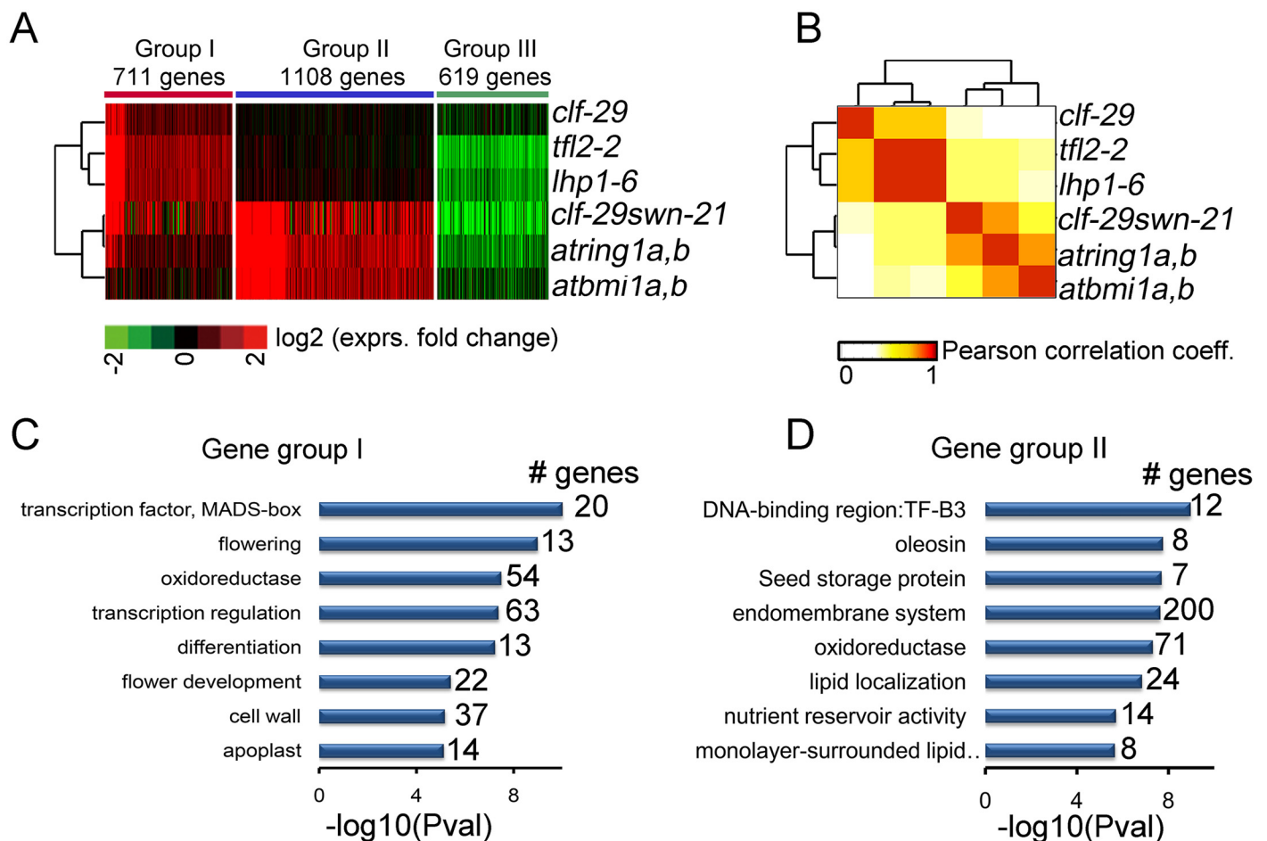
Fig 4. The profile of transcriptome change reveals two distinct combinations of PcGs with different functions. Three groups of genes showing distinct expression change profiles across mutants of PcG components. Green and red colors represent lower and higher expression in PcG mutants. Heatmap including another 1,290 genes whose expression affected only in clf-29swn-21 is shown in S5A Fig. RNA-seq data sets were clustered via unsupervised hierarchical clustering based on Pearson correlation coefficients of log 2 expression fold-change across samples. (C-D) Functional terms enriched in genes from group 1 (C) and group 2 (D) as shown in (A).
