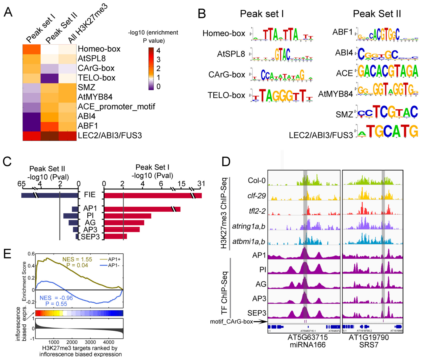
Fig 6. TF binding motifs and TFs whose bindings are enriched in peak set I and peak set II. (A) Heatmap showing enriched motifs (P value < 0.01) in either peak set I or peak set II. Their enrichment in H3K27me3 peaks in Col-0 are also shown. (B) Sequence LOGOs of motifs enriched in peak set I and peak set II. (C) Enrichment of the binding sites of FIE and TFs in peak set I. (D) IGV screen shots showing examples of co-occupancy between H3K27me3 in seedlings and the bindings of MADS-box TFs in inflorescence. The motif sites of MADS box TFs are indicated by pink and blue bars at bottom of the screen shots, and are highlighted by grey area. (E) GSEA showing the common target genes of peak set I and AP1 binding peaks are preferentially expressed in inflorescence.
