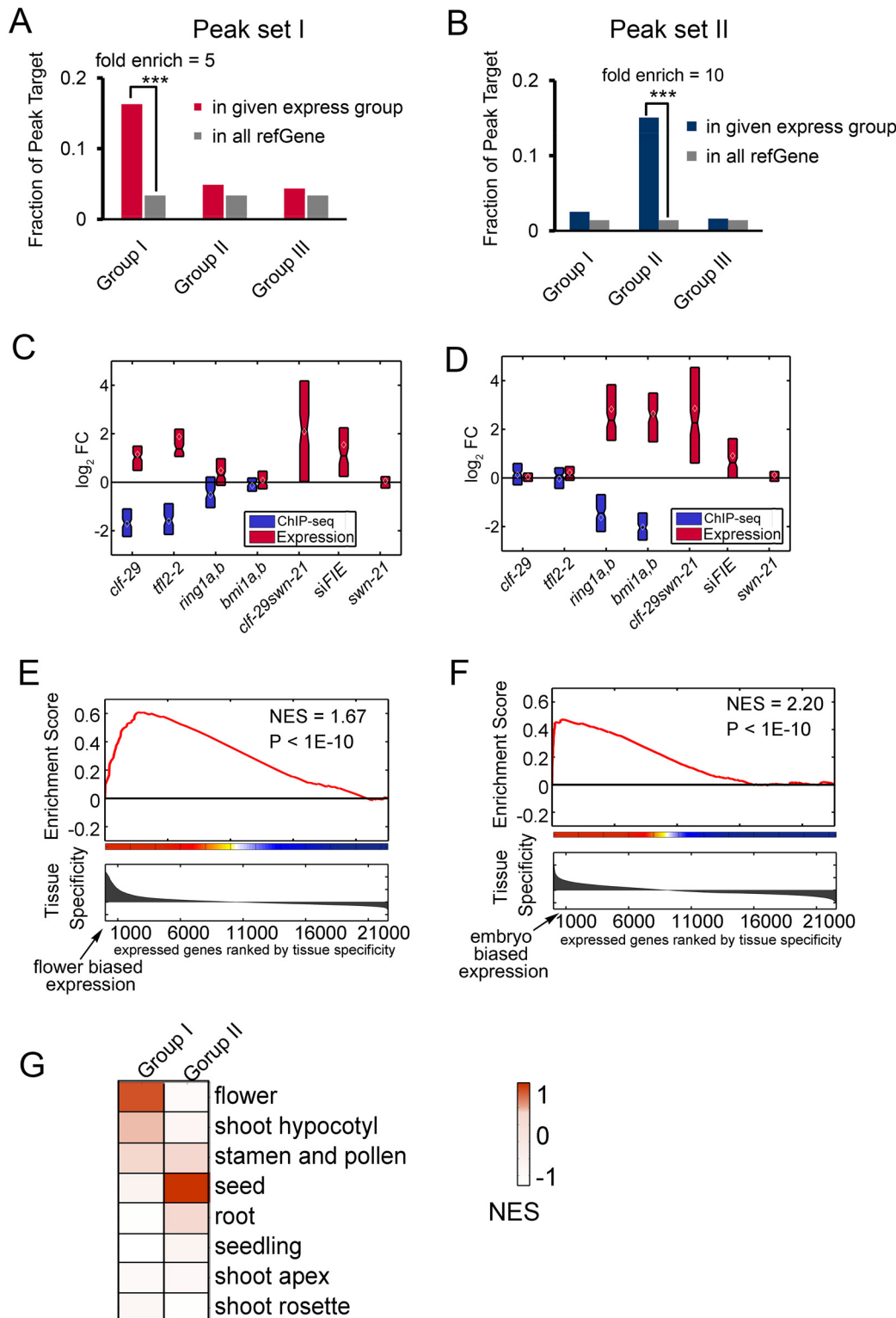
Fig 5. Targets of different combinations of PcGs and their expression bias. (A) Enrichment analysis of peak set I targets in three expression groups shown in Fig 4A. ***, Fishers' exact test P value < 1e-3. (B) Enrichment analysis of peak set II targets in three expression groups shown in Fig 4A. ***, Fishers' exact test P value < 1e-3. (C-D) Box plot showing the distribution of expression changes and H3K27me3 changes for 108 genes (C) and 164 genes (D) in PcG mutants. (E-F) Gene Set Enrichment Analysis (GSEA) showing a significant normalized enrichment score (NES) for flower biased expression of 108 genes (E) and embryo biased expression of 164 genes (F). The x axis represents all expressed genes ranked by tissue specificity as determined by
