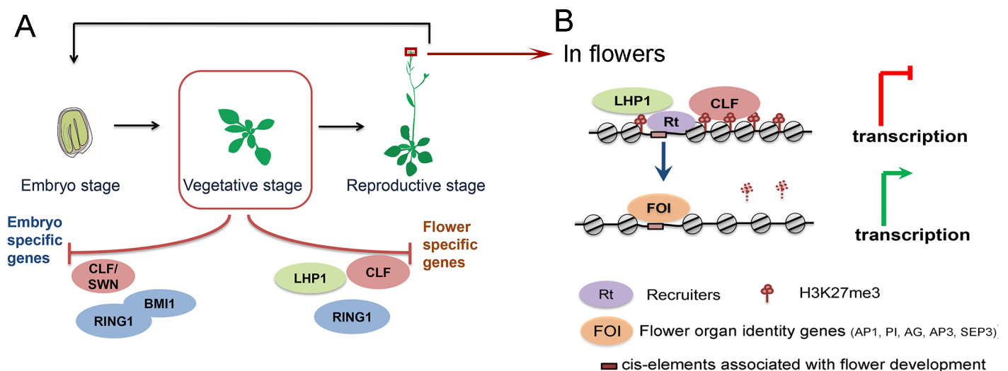
Fig 7. Working model for specific regulation of plant development by PcG components. (A) In seedlings, CLF and LHP1 work concertedly to repress flower specific genes, and some targets are also regulated by RING1. While repression of embryonic development requires cooperative regulation of AtBMI1, AtRING1, and the redundant role of CLF and SWN. (B) In inflorescence, significant parts of CLF and LHP1 target sites in seedlings are occupied by inflorescence specific TFs, which participate in de-repression of the common target genes.
