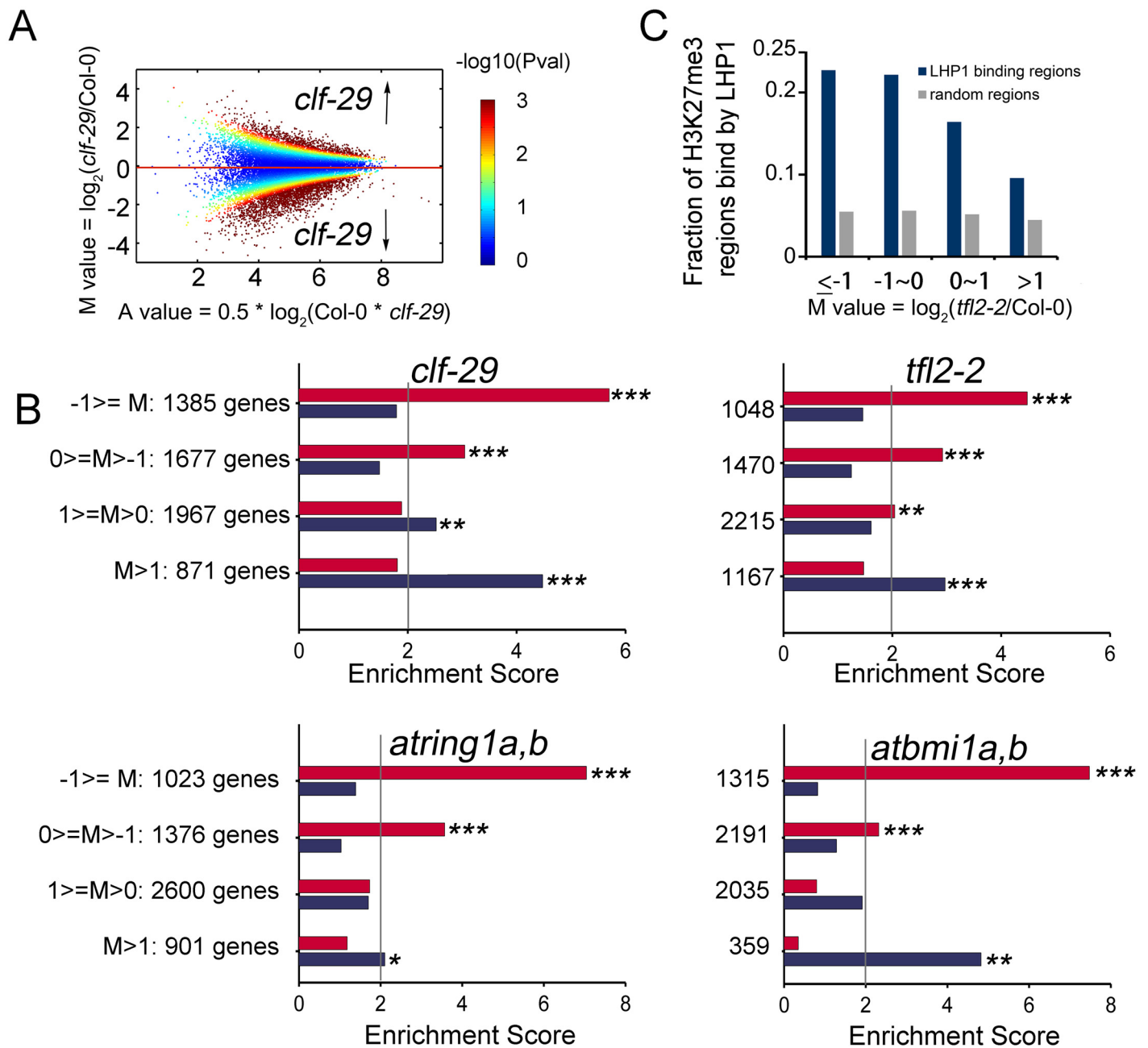
Fig 2. Quantitative difference of H3K27me3 marks are inversely correlated with the change of target gene expression in PcG mutants. (A) MA plot of all peaks from comparison of clf-29 and Col-0 after normalization by MAnorm. Each dot represents a peak. X-axis is the A value, which represents the average intensity. Y-axis is the M value, which represents the difference of the intensity. Here, positive M value indicates higher H3K27me3 level in clf-29 as compared to that in Col-0, and negative M value represents lower H3K27me3 level in clf-29 . The color range represents -\log_{10} P value associated with normalized peaks. (B) Enrichment of H3K27me3 peak targets with different M values in gene sets whose expression are regulated by different PcGs. The target genes were grouped by the M values of nearby peaks. For each group, the overlap with differentially expressed genes in a given PcG mutant was compared to the expected overlap at random; x-axis represents enrichment score. Fishers' exact test was used to test the significance of overlap. *, P value < 5e-2 ; **, P value < 1e-2 ; ***, P value < 1e-3 . (C) Bar plot showing the percentage of H3K27me3 peaks with different M values in tff2-2 overlapped with LHP1 binding sites.
