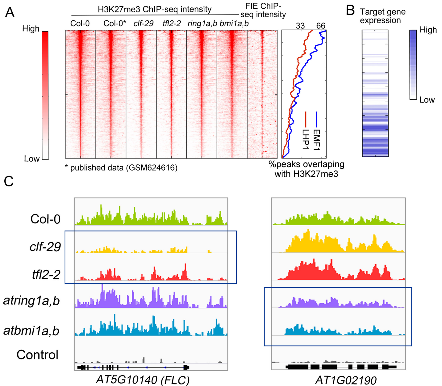
Fig 1. Local difference of H3K27me3 marks in mutants of PcG components. (A) ChIP-seq density heatmaps in Col-0 and PcG mutants, ranked by H3K27me3 read intensity within \pm 500 bp of peak summits in Col-0. The Pearson correlation coefficient between H3K27me3 intensity in Col-0 and FIE binding within \pm 50 bp of peak summits is 0.52. ChIP-seq data of H3K27me3 in panel II and FIE binding in panel VII were published previously [40,41]. To compare H3K27me3 level with the bindings of LHP1 and EMF1 based on published ChIP-chip data [15,32], the fraction of EMF1 peaks (blue) or LHP1 peaks (red) Col-0 overlapped with Col-0 H3K27me3 peaks were plotted. (B) RNA-seq intensity heatmap for the targets of H3K27me3 peaks in Col-0 with the same order as in (A). The expression intensity is measured by Reads Per Kilobase per Million of mapped reads (RPKM). (C) IGV screen shots showing the distribution of H3K27me3 mark intensity in Col-0 and different mutants of PcG components. Negative control is Col-0 sample immunoprecipitated with beads but without antibody. Regions showing quantitative reduction of H3K27me3 marks are highlighted by blue box.
