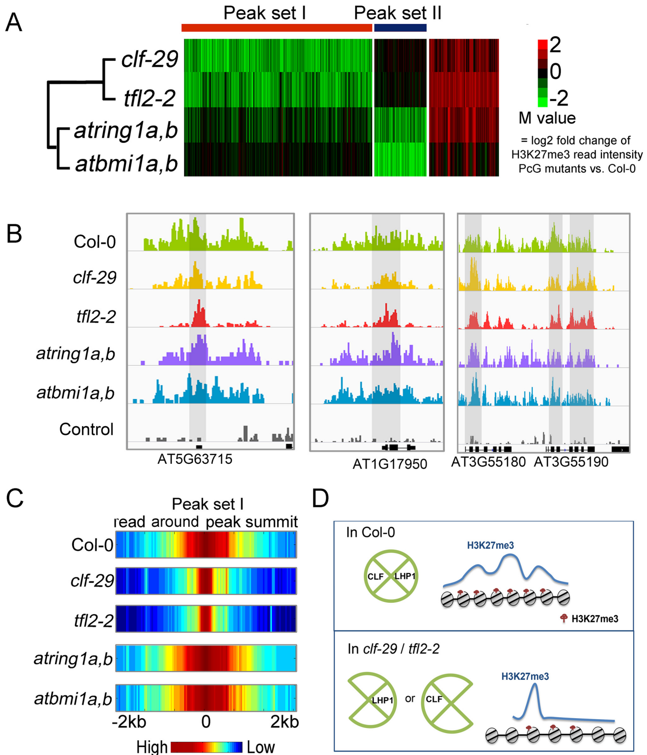
Fig 3. clf-29 and tfl2-2 show coordinated H3K27me3 change profiles distinct from those in ating1a,b and atbmi1a,b . K-means clustering of M values characterizing the quantitative change of H3K27me3 in PcG mutants. Definition of H3K27me3 quantitative change regions were based on combined criteria |M| > 1 and P \text{ value} < 1e-3 . Green and red colors represent lower and higher H3K27me3 levels in PcG mutants compared to that in Col-0. IGV screenshots support CLF and LHP1 participate in H3K27me3 elongation. Grey areas represent regions where significant H3K27me3 reductions happen mainly in surrounding regions but not in summit regions in tfl2-2 and clf-29 compared to Col-0. It's worth noting that no smooth should be applied while preparing data
