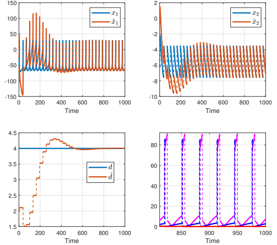
Fig. 4. Top and bottom left : jump-based estimation of (x_1, x_2, d) in the neuron model (44) without delay. Bottom right : norm of the residual estimation error without delay (red), with delay \Delta = 1 (blue), with delay \Delta = 5 (pink).
