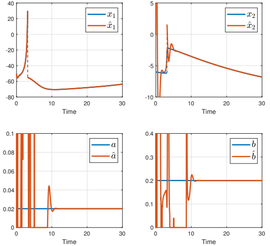
Fig. 3. Flow-based estimation of (x_1, x_2, a, b) in the neuron model (44) through high-gain observer.
