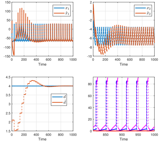
Fig. 3. Top and bottom left : jump-based estimation of (x_1, x_2, d) in the neuron model (40) without delay. Bottom right : norm of the residual estimation error without delay (red), with delay \Delta = 1 (blue), with delay \Delta = 5 (pink).
