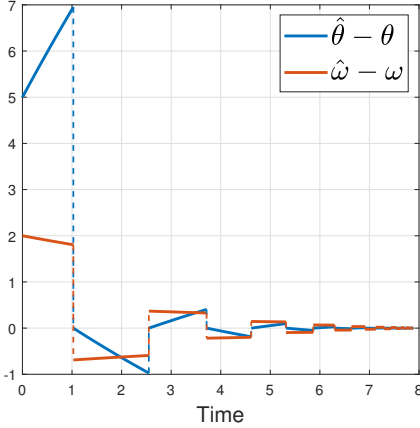
Fig. 1. Jump-based estimation of a Zeno bouncing ball (39).
