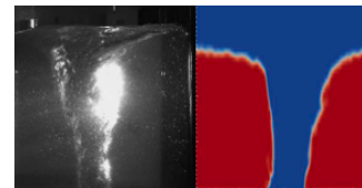
FIGURE 2 – Experimental and numerical bathtub vortex
