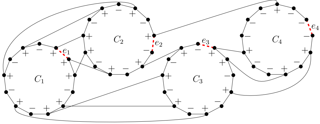
Figure 5: An illustration of the odd cycles \{C_1, C_2, C_3, C_4\} from a 2-factor considered in proof of Proposition 3.6 (dashed lines: edges of A ; the edge having end vertices labeled by - in G - \mathcal{F} are omitted in order to simplify the figure).
