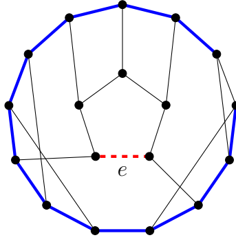
Figure 4: An edge e at distance at most 3 of twelve edges from a 13-cycle (dashed line: e ; thick lines: edges at distance at most 3 from e in the 13-cycle).
