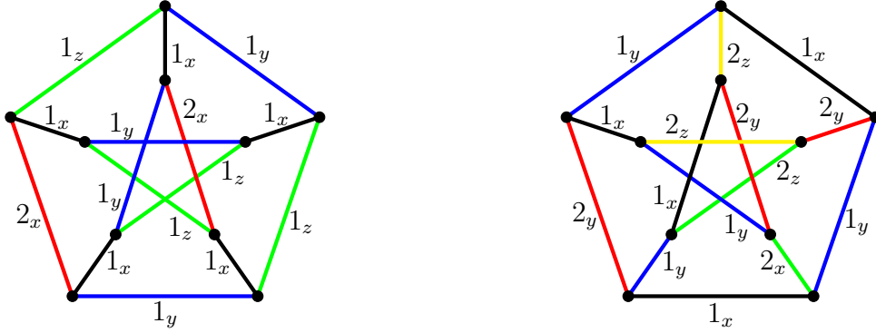
Figure 1: A (1, 1, 1, 2) -coloring (on the left) and a (1, 1, 2, 2, 2) -coloring (on the right) of the Petersen graph.
