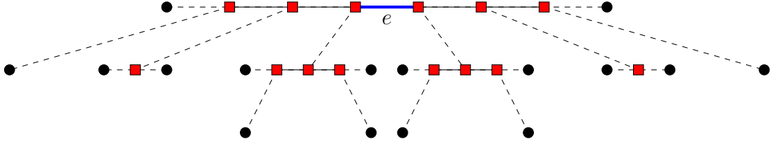
Figure 3: The vertices at distance at most 2 of an edge e and the set D_e^3 (dashed or non dashed line: edge at distance at most 3 from e ; square: vertex in D_e^3 ; non dashed line: edge in D_e^3 ; horizontal line: edge in \mathcal{F}' ).
