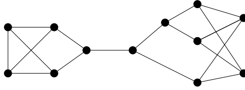
Figure 6: The smallest non (1, 1, 2, 2, 2) -colorable and non (1, 2^6) -colorable cubic graph.
