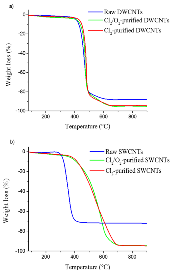
Figure 2. TGA curves (in dry air, temperature ramp 5 °C/min) for the raw and selected CNTs treated with \text{Cl}_2 and \text{Cl}_2/\text{O}_2 (a): raw DWCNT rD (blue); \text{Cl}_2 -purified DWCNT D3 (red); \text{Cl}_2/\text{O}_2 -purified DWCNT D1 (green) and for SWCNTs (b): raw SWCNT (blue) rS1-2; \text{Cl}_2 -purified SWCNT S5 (red); \text{Cl}_2/\text{O}_2 -purified SWCNT S1 (green).
