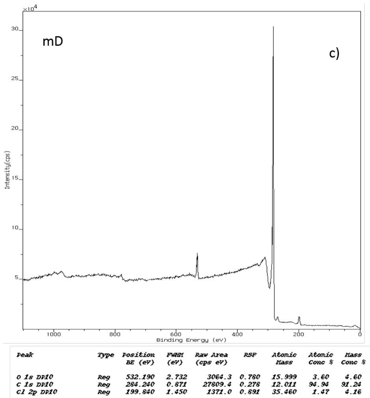
Fig. S5. XPS wide scans of a) rD, b) D1 and c) mD.
