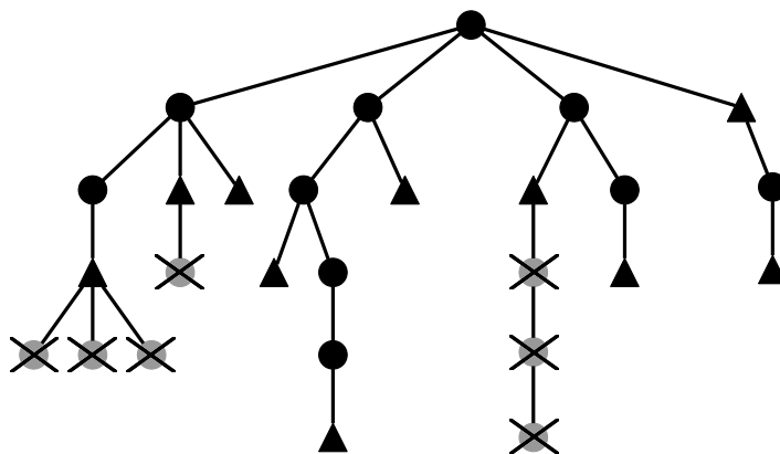
Figure 16: Deletion of non-terminal leaves.
