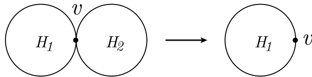
Figure 14: Deletion of useless components.
