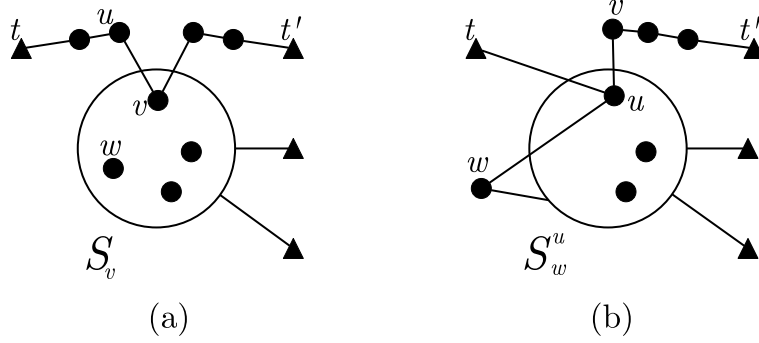
Figure 3: Two separators S_v and S_w^u .
