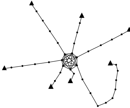
Figure 7: Clique star of 7 terminals.
