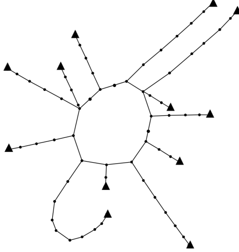
Figure 11: Extended terminal cycle with \beta(J) = 2 .
