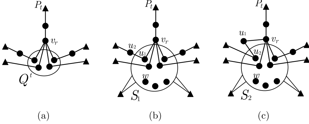
Figure 5: A ring Q^t and two separators S_1 and S_2 .
