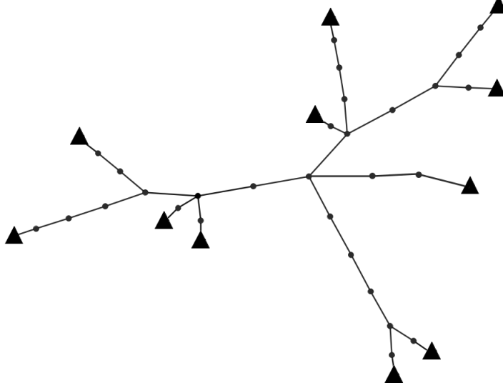
Figure 9: Terminal tree of 10 terminals.
