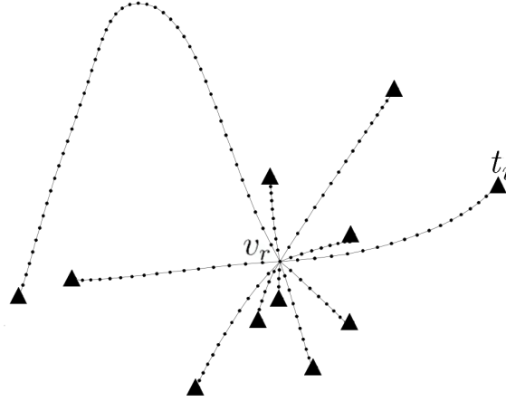
Figure 4: A Star tree.
