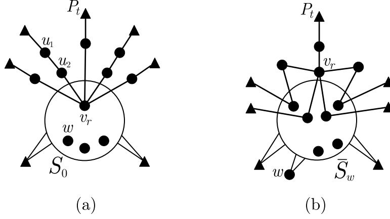
Figure 6: Two separators S_0 and \bar{S}_w .
