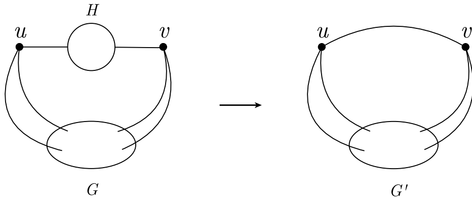
Figure 13: Contraction of a subgraph connected to two vertices.
