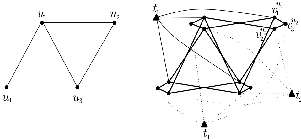
Figure 2: Transformation from the graph H to the graph G .
