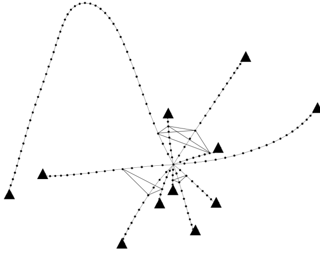
Figure 8: Star tree with clique branches.
