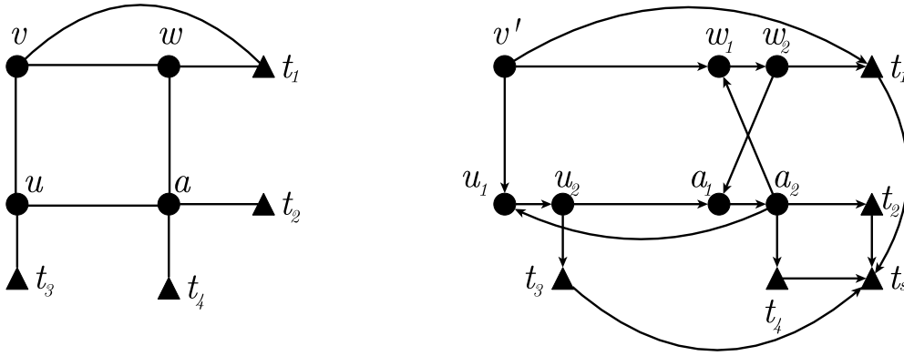
Figure 15: Transformation graph from G to D_v
