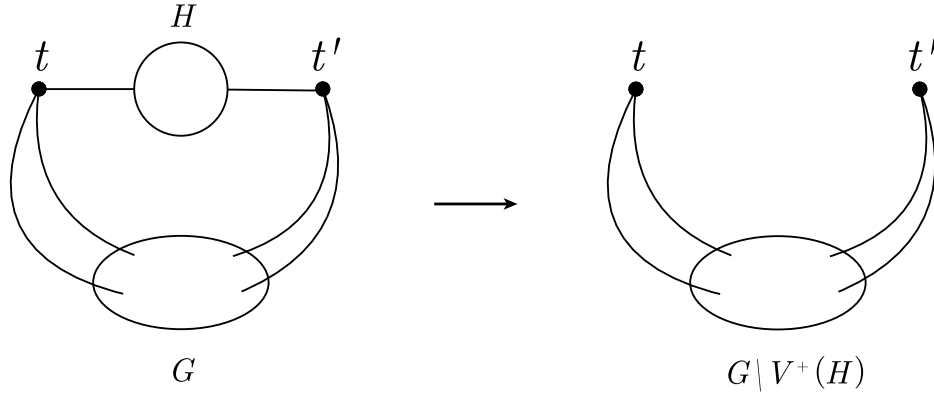
Figure 12: Deleting a subgraph connected to two terminals.
