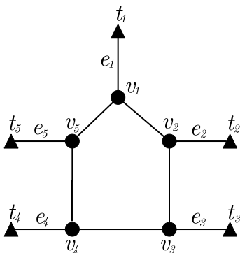
Figure 10: Terminal cycle of 5 terminals.
