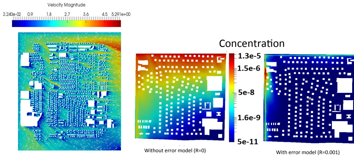
FIGURE 5 – Wind field corresponding to conditions over Fresno on April 1, 2001 (left). Dimensionless concentration with two pollution sources solution (right).
