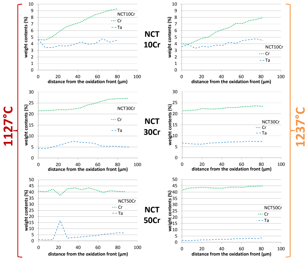
FIGURE 5. Concentration profiles in the subsurfaces of three of the five alloys after oxidation at 1127°C and at 1237°C (SEM/EDS)
