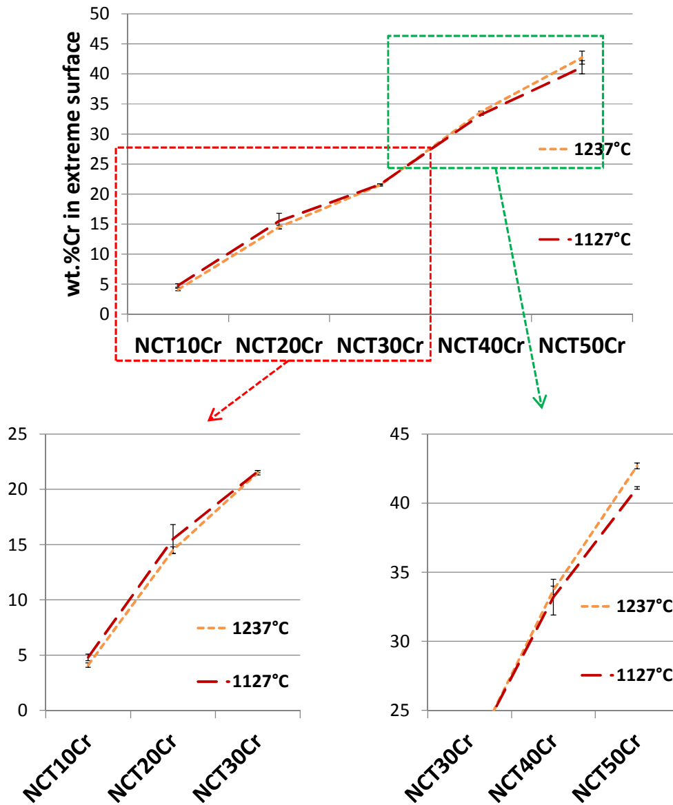
FIGURE 8. Comparison between the chromium content in extreme surface after 24h of oxidation at 1127°C and at 1237°C (SEM/EDS)
