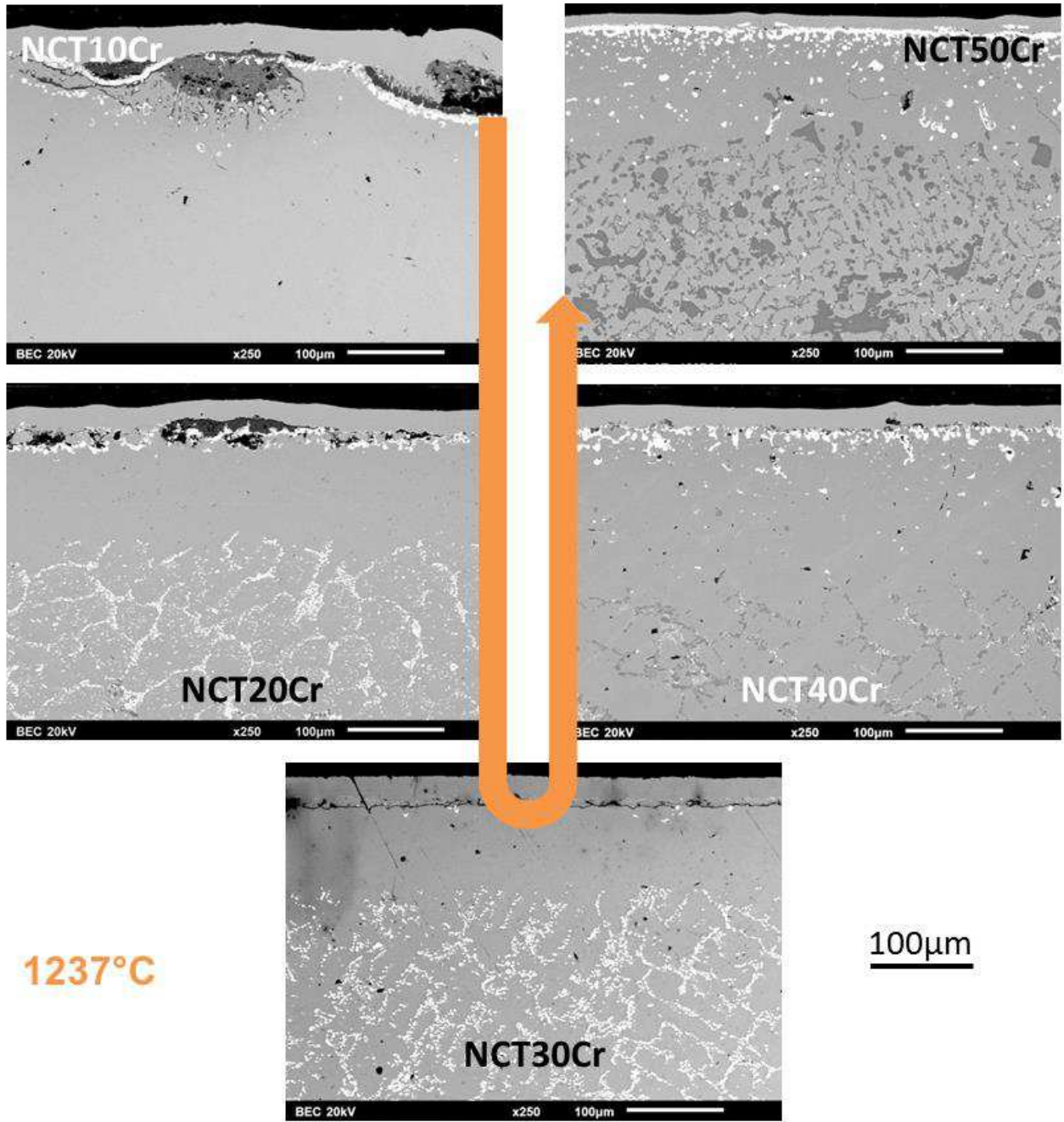
After oxidation at 1237°C: general view (×250)
