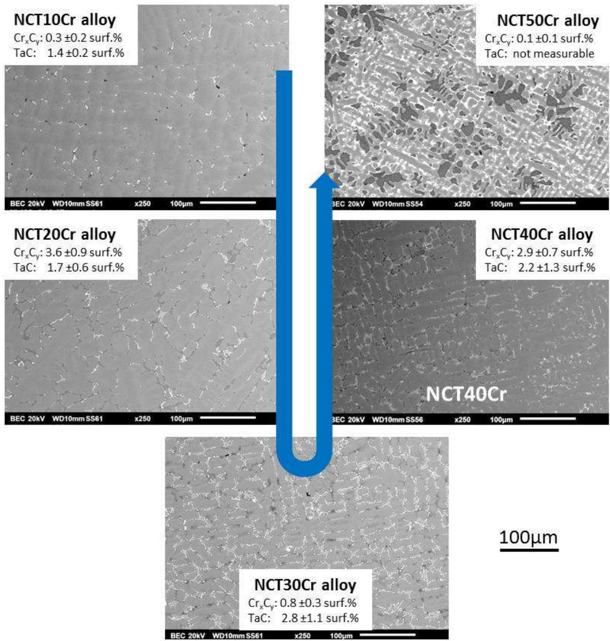
As-cast microstructures: general view ( \times 250 )
