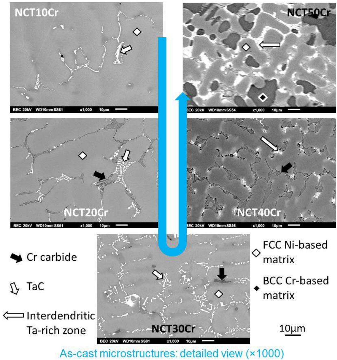
FIGURE 2. As-cast microstructures of the five studied alloys (SEM/BSE micrographs, detailed view, ×1000)
