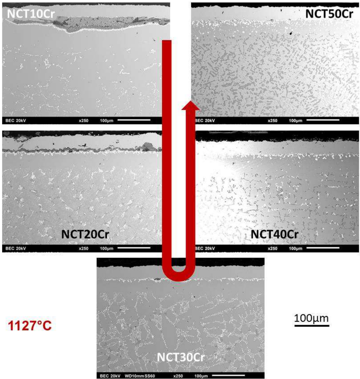
After oxidation at 1127°C: general view (×250)
