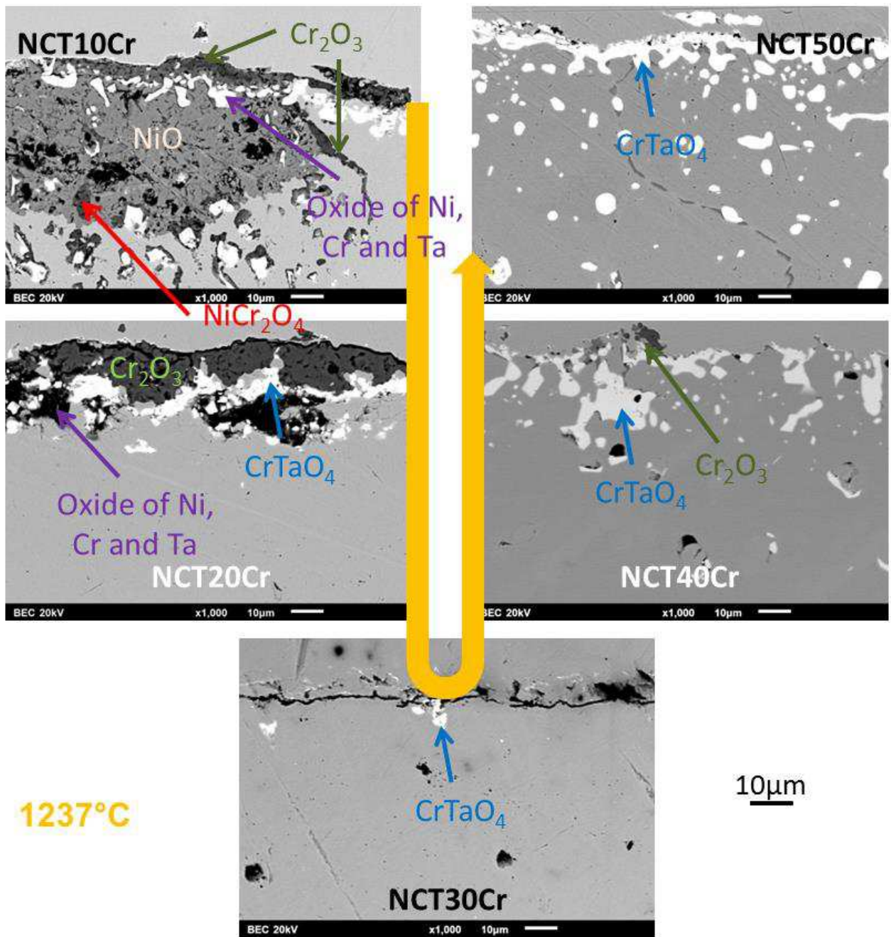
After oxidation at 1237^\circ\text{C} : detailed view ( \times 1000 )
