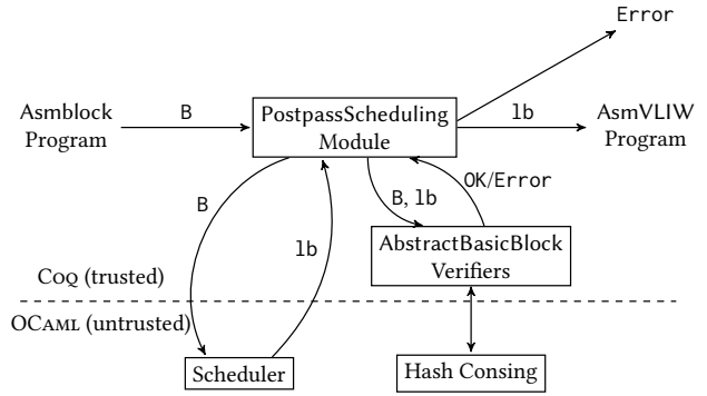
Fig. 6. Certified Scheduling from Untrusted Oracles
