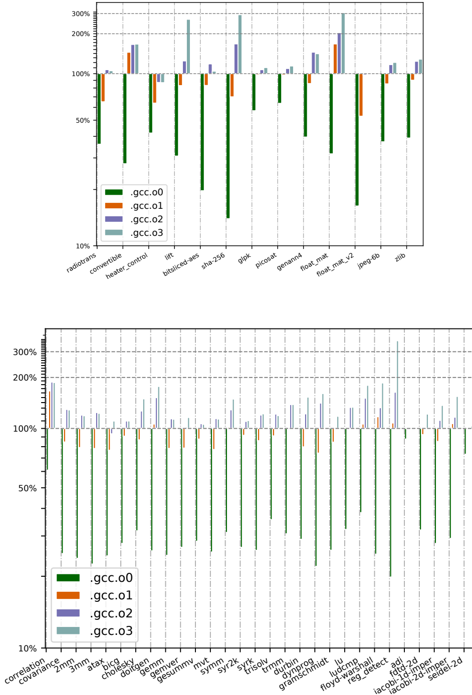
Fig. 17. Relative Speed of Generated Code with Kalray’s GCC, from -O0 to -O3 Optimization Levels; 100% being the Speed with COMP CERT by List Scheduling (Lower is Slower). Note that for some safety-critical applications with mandatory traceability from source to object code (e.g., DO178 level-A avionics), only gcc -O0 is likely to be usable, whereas COMP CERT’s correctness proof is accepted for traceability [Bedin França et al. 2012]. Our target benchmark is pictured at the top, Polybench is at the bottom picture.
