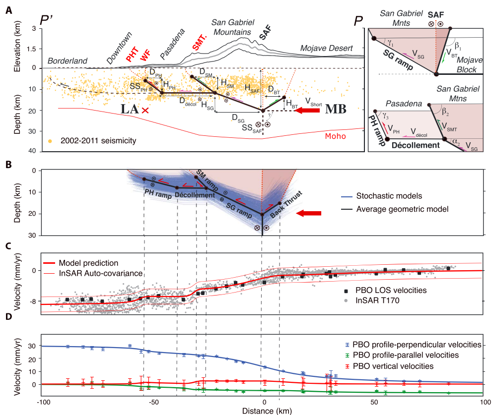
Figure 2. Comparison between the prior and posterior models. (a) Two-dimensional prior model based on the tectonic review along the profile PP' defined in Figure 1. Black lines (red dashed lines, respectively) represent slipping (locked, respectively) sections of the faults; arrows indicate relative direction of the movement on faults. The SAF is associated with two thick black dashed lines and a question mark as we have no constraints of its deep geometry. We use this configuration and the conservation of motion along each junction to explore the various parameters defined in this figure. Insert is a simplified two-dimensional block model illustrating the relation between the block geometries and longitudinal velocities along the structures. (b) Posterior geometries in agreement with the data (blue lines) and average geometry (black lines). (c) InSAR LOS velocities (grey points) and GPS projected in the LOS direction (black squares) and average model obtained. (d) Profile-perpendicular (blue markers), profile-parallel (green markers), and vertical (red markers) GPS velocities with their associated uncertainties. Average model obtained (blue, green, and red lines) along profiles.
