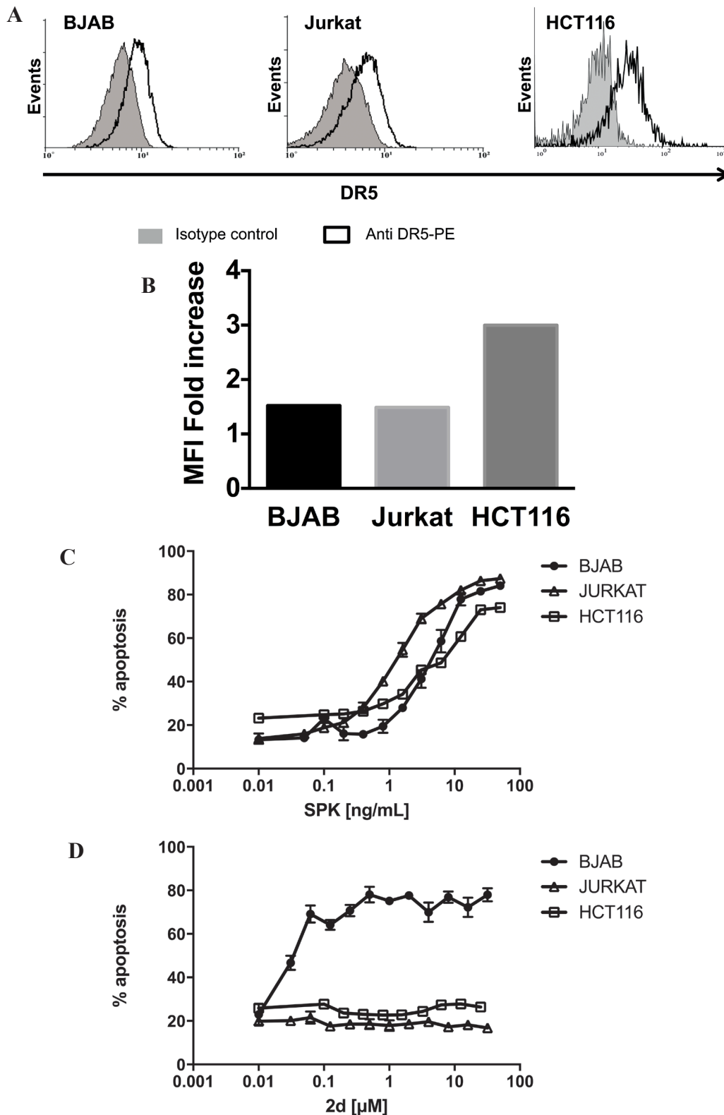
Figure 1: Differential apoptogenic activity of SPK and TRAIL min /DR 5 . BJAB Jurkat and HCT116 cells A. were stained with monoclonal antibody directed against DR5 or a control isotype coupled to phycoerythrin (PE) and analyzed by flow cytometry. Results in B. showed fold increase of the mean of fluorescence intensity between control isotype and TRAIL-R2 specific labeling that was calculated to compare level of TRAIL-R2 expression on the three cells lines. BJAB, Jurkat and HCT116 cells were treated with stepwise 2-fold increasing concentrations of SPK C. or divalent TRAIL min /DR 5 peptide (2d) D. After 16 hours of incubation, apoptosis was determined as the percentage of Annexin V-positive cells by flow cytometry analysis. Results are expressed as mean % apoptosis of 3 independent experiments +/- SD.
