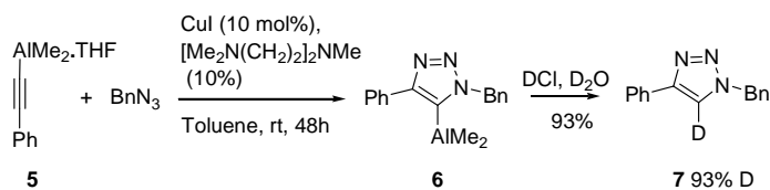
Scheme 1. Deuteration study.
