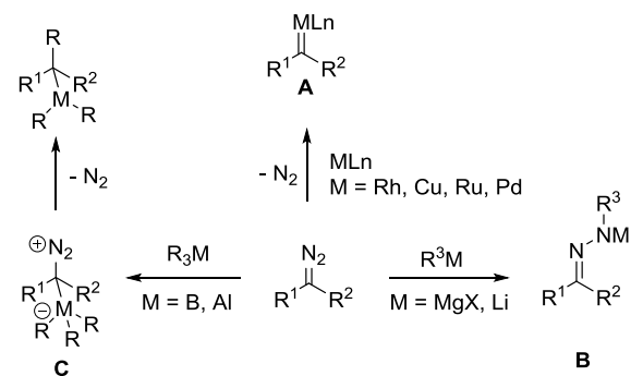
Figure 1. General reactivity of diazocompounds with organometallic reagents
