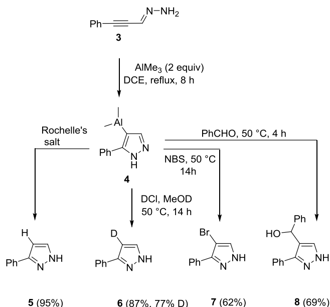
Scheme 4. Synthesis of NH -pyrazoles from 3
