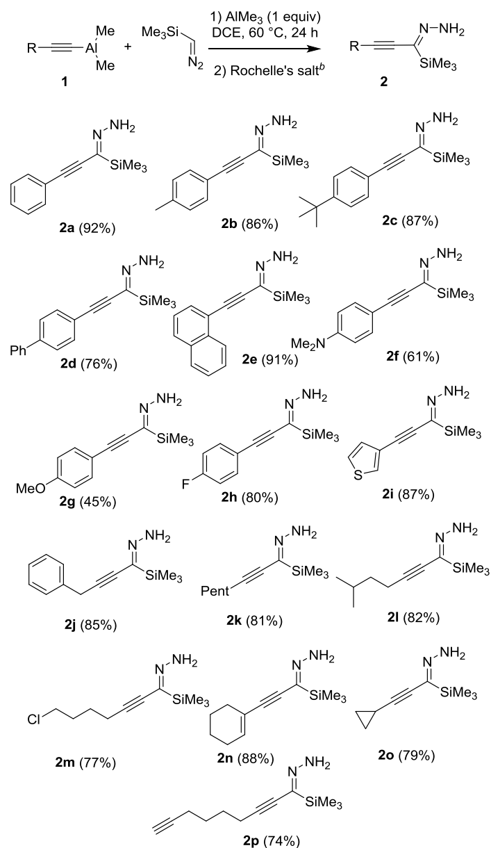
Scheme 1. Scope of the reaction a
