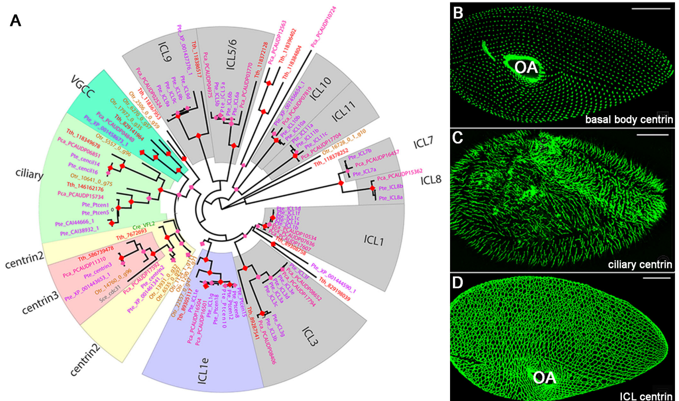
Fig. 1. Ciliate centrans: phylogeny and localisation in Paramecium . (A) Maximum-likelihood unrooted tree of ciliate centrans. The robustness of the nodes is coded by coloured diamonds: pink for aLRT scores superior to 75%, red for aLRT scores superior to 95%. Boxes indicate well supported sub-groups, from either the phylogenetical or functional point of view. Pte (purple): Paramecium tetraurelia ; Pca (pink): Paramecium caudatum ; Tth (red): Tetrahymena thermophila ; Otr (brown): Oxytricha trifallax . Two outgroup sequences for Centrin2 and Centrin3 families have been added: Cre/VFL2 (green), Chlamydomonas reinhardtii and Sce/cdc31 (grey), Saccharomyce cerevisiae . (B-D) Confocal images. GFP-tagging of representatives of these diverse centrans reveals their three major localisations: at basal bodies (B), in cilia (C) and along the infraciliary lattice (D) labelled by GFP-Centrin2, GFP-Cent14 and GFP-ICL1e, respectively. OA, oral apparatus. Scale bar: 20 µm.
