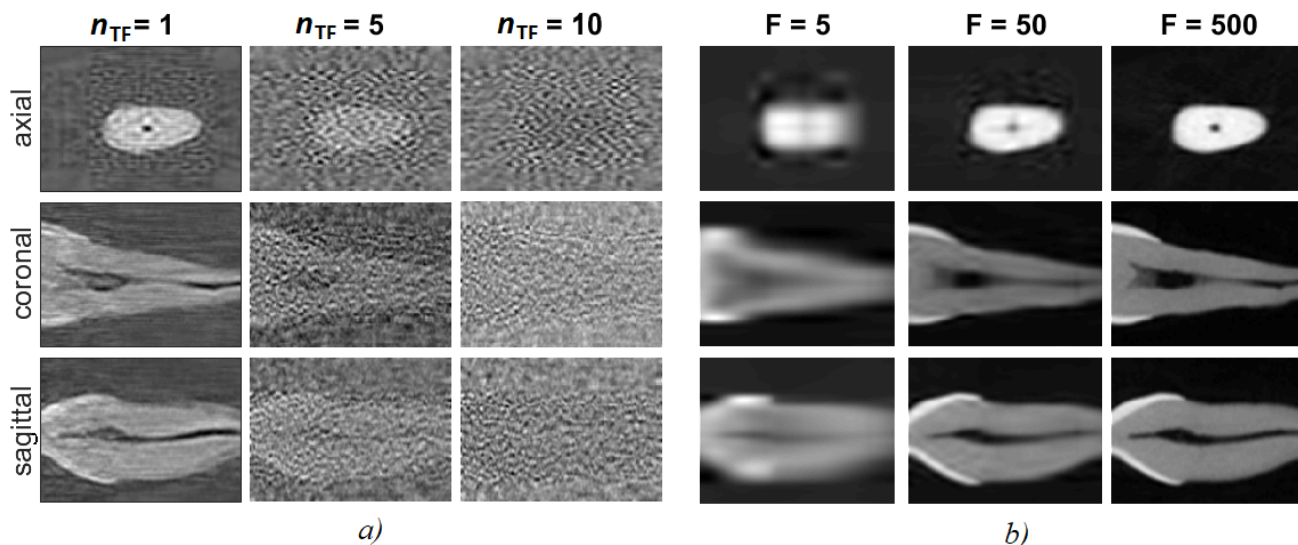
Fig. 6. Effect of the iteration number it and the tensor rank F in the reconstructed images. Sample #1 is visualized through 3 slices from the axial, coronal and sagittal directions. In panel a) the difference compared to a result obtained after 10 iterations is shown. In case of n_{TF}=10 , a second test run was used for calculating the difference (note that the algorithm has random initialization, therefore different runs result in slightly different outputs). With more iterations the difference becomes less structured, more random. In panel b) the change with F can be seen: low numbers cause large blocks in the images, and the higher the tensor rank, the more detailed the output is.
