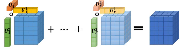
Fig. 1. Illustration of tensor factorization. F is the number of outer products formed by mode-1 ( U^1 := U^1(:, i) ), mode-2 ( U^2 := U^2(:, j) ) and mode-3 ( U^3 := U^3(:, k) ) fibers summing up to a rank- F tensor.
