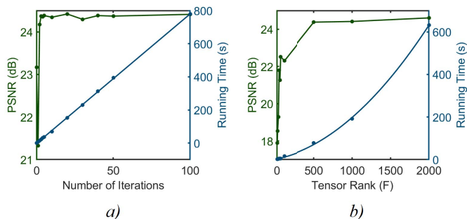
Fig. 7. Effect of the iteration number and the tensor rank on the PSNR and runtime. The rest of the parameters are as in Table I. In a) the PSNR saturates after a small number of iterations, while the runtime increases linearly. In b) the runtime has an exponential growth versus the tensor rank and the PSNR saturates around F = 500 .
