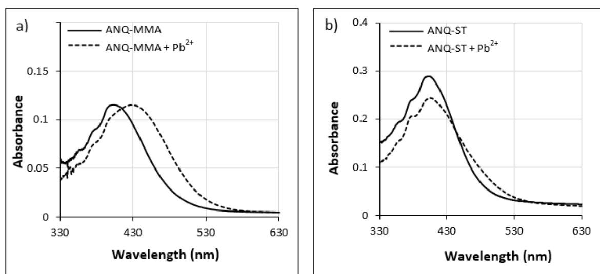
Fig. 1. Absorbance spectra of a) ANQ-MMA and b) ANQ-ST ( 50 \mu\text{mol.L}^{-1} ) in acetone-water (4:1, v/v) solution and in presence of 100 \mu\text{mol.L}^{-1} of \text{Pb}^{2+} .
