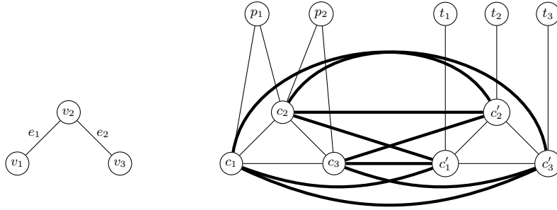
Fig. 3. Construction of split graph H = (V_H, E_H) from a P_3 . The weights of thick edges in H are 1 and for the others are 0.
