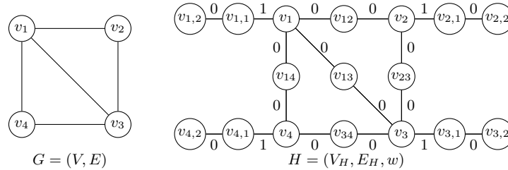
Fig. 2. Construction of H from G . The weights are indicated on edges.
