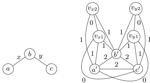
Fig. 4. The constructed weighted graph G' = (V', E'.w) (right side) build from a P_3 G = (V = \{a, b, c\}, E = \{1, 2\}) (left side).
