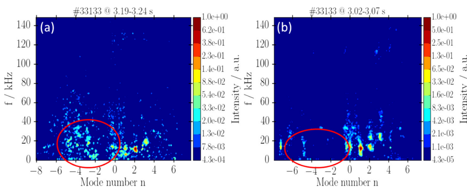
FIG. 8. Experimental mode spectrum in ELM mitigation (a) and ELM suppression (b) phases of the discharge #33133: the intensity of the modes is plotted depending on their frequency and toroidal mode number.
