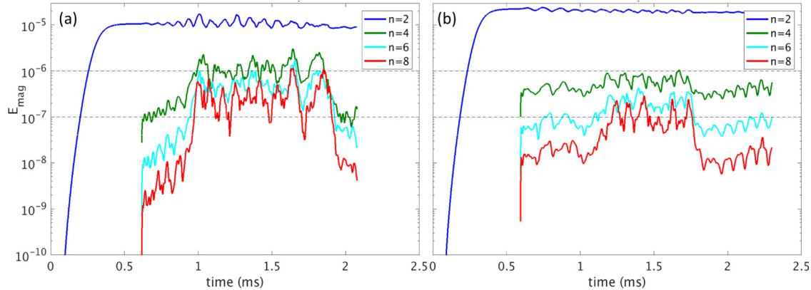
FIG. 5. Magnetic energy of the modes n=2 , 4, 6, and 8 in the ELM mitigation case obtained for nominal RMP amplitude (a) and in the ELM suppression case obtained at RMP amplitude increased by 50% (b).
