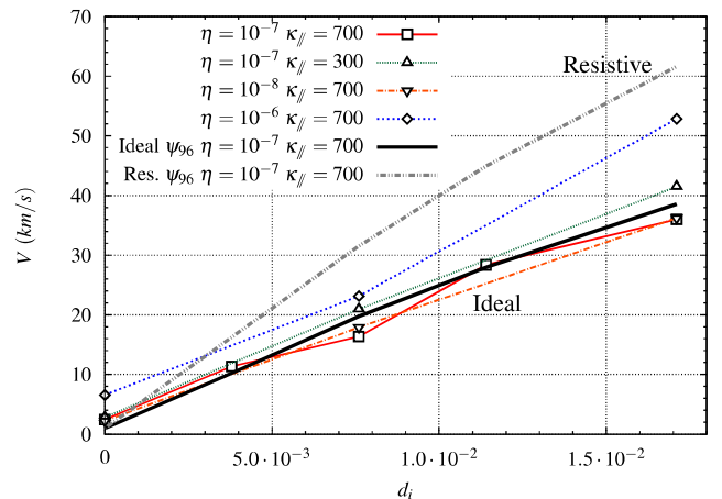
FIG. 3. Poloidal rotation velocity of the modes as a function of d_i and comparison with the expressions Eqs. (4) and (5) taken at \Psi_{96} (i.e., at the flux surface with |\nabla P|_{max} ), \kappa_{\parallel} is the normalized parallel heat conductivity.
