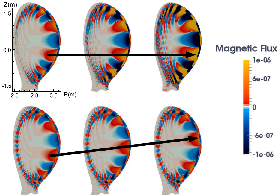
FIG. 2. Magnetic flux perturbation n=6 , same parameters as in Ref. 25 ( 10\ \mu\text{s} between images) (top) without diamagnetic effects, d_i=0 and (bottom) with diamagnetic effects, d_i = 1.7 \times 10^{-2} . In the bottom, the rotation is anticlockwise, i.e., in the electron diamagnetic or \mathbf{E} \times \mathbf{B} direction.
