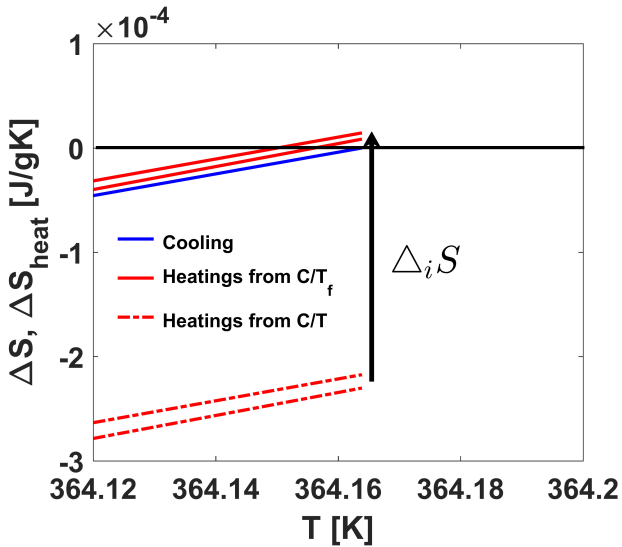
FIG. 11: Configurational entropy of PVAc obtained by integration of C_i/T and C_i/T_f as a function of temperature during cooling and the successive heating for the experiments 1 and 2 such as described in table I. The figure shows a magnification of the configurational entropy in the temperature range around the starting and final temperature.
