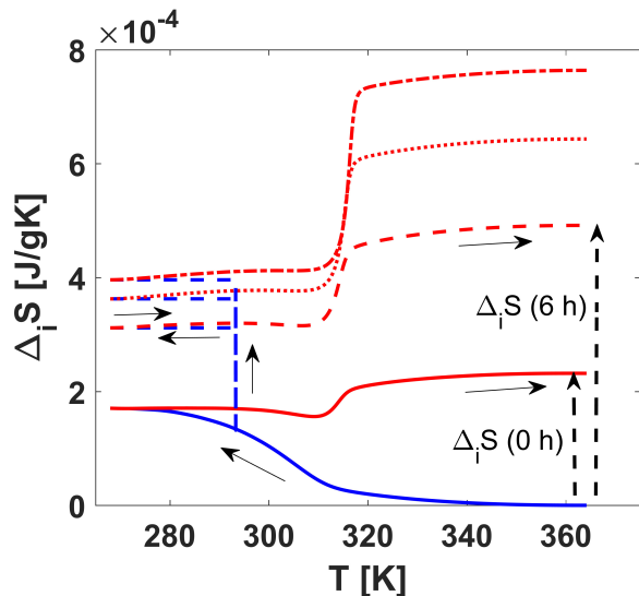
FIG. 12: Entropy production contributions for PVAc as a function of temperature during different parts of the thermodynamic cycles for the experiment 1 during cooling and the successive heating, and for the experiments 3, 4 and 5 during cooling, during annealing, during the rest of cooling, and during the successive heating such as described in table I. The black arrows indicate the sense of progression of the thermodynamic cycle for the experiment 5 with 6 h of aging at 293.3K.
