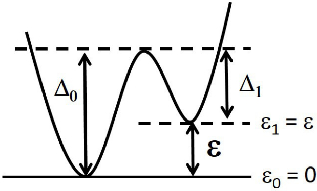
FIG. 1: Double-well potential of a two-level-system.
