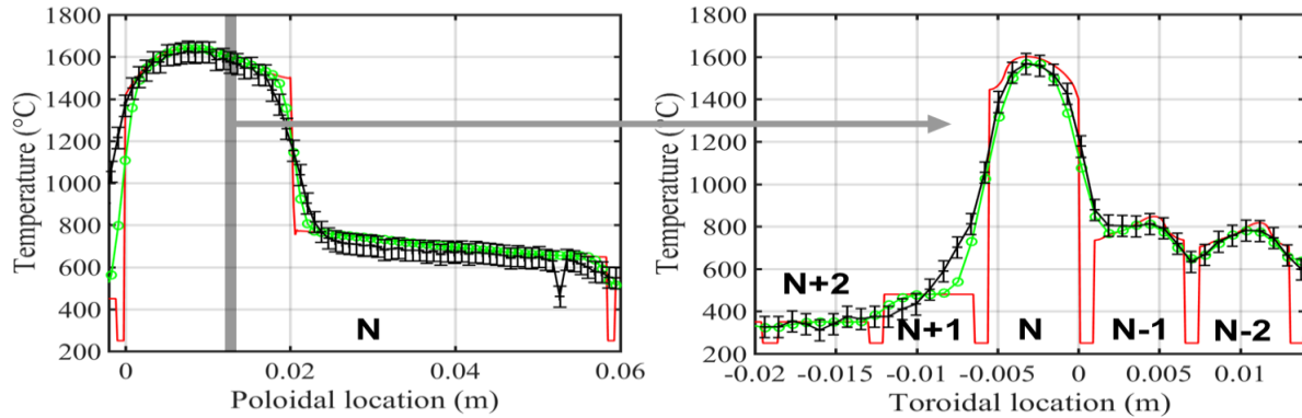
Figure 5. (—) ANSYS, (—) synthetic IR data and (—) IR data. (left) poloidal and (right) toroidal temperature profiles @ t = 12.048\text{s} before the ELM crash.
