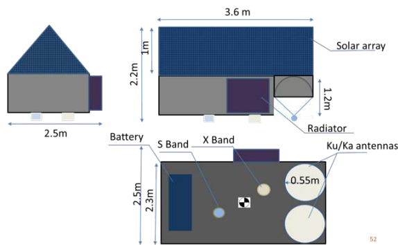
Figure 7: Spacecraft design
